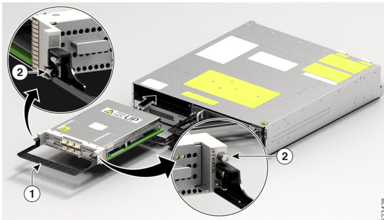
Figure 10: Inserting the NCS1K14-2.4T-K9 Line Card
