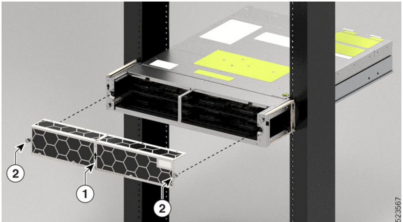
Figure 22: Installing the Air Filter
