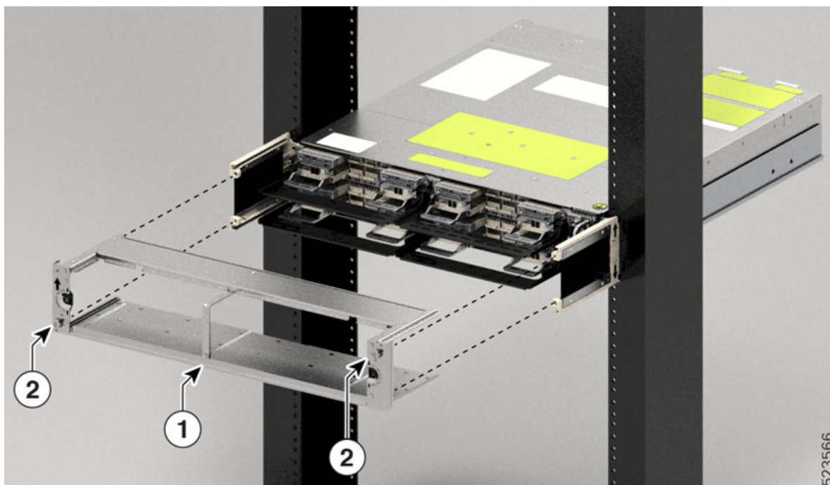
Figure 21: Installing the Air Filter Frame
