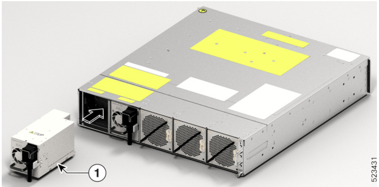
Figure 13: Inserting the PSU
