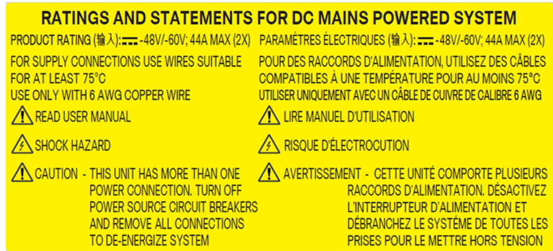
Figure 14: Rating Label for DC Power
