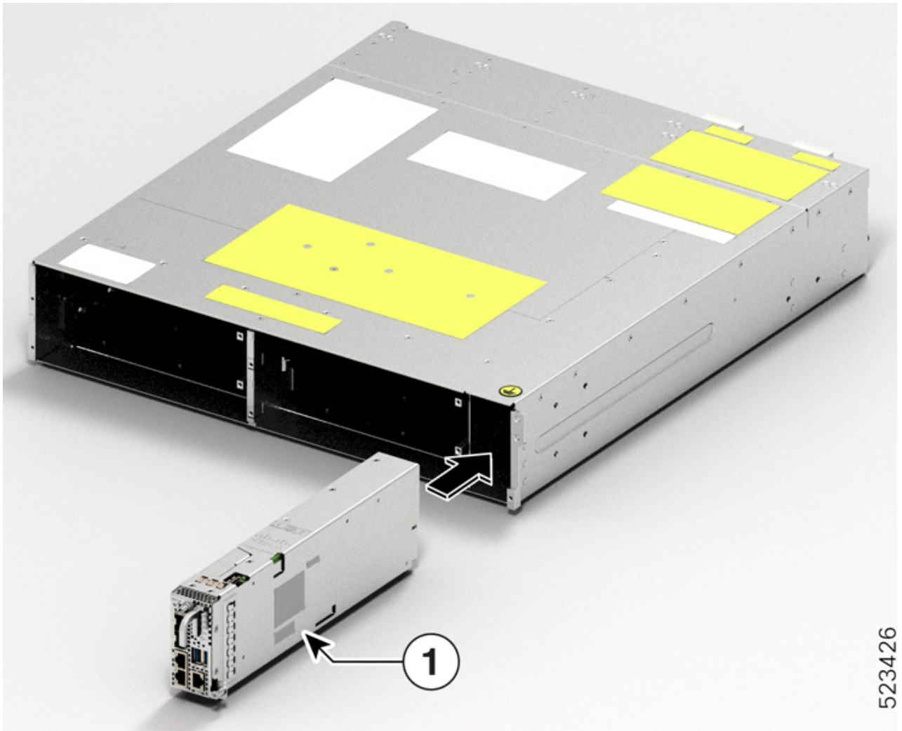
Figure 6: Inserting the Controller
