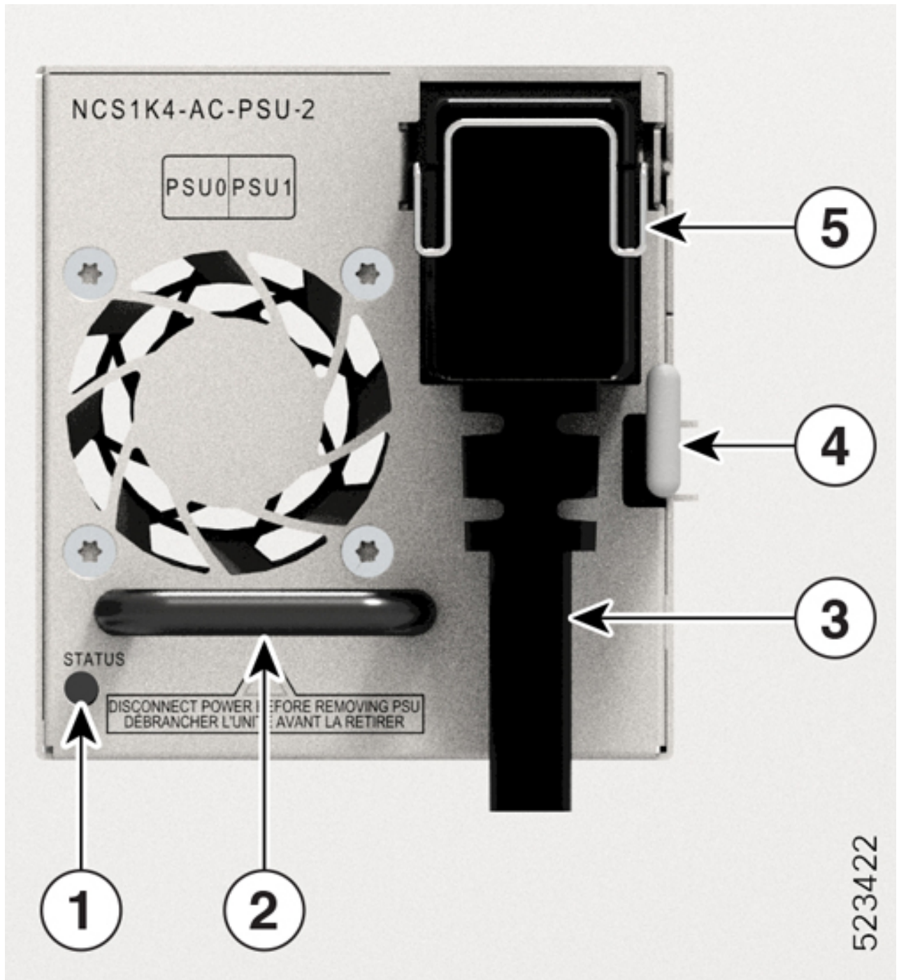
Figure 17: NCS1K4-AC-PSU-2 with 180-Degree Cable Connection
