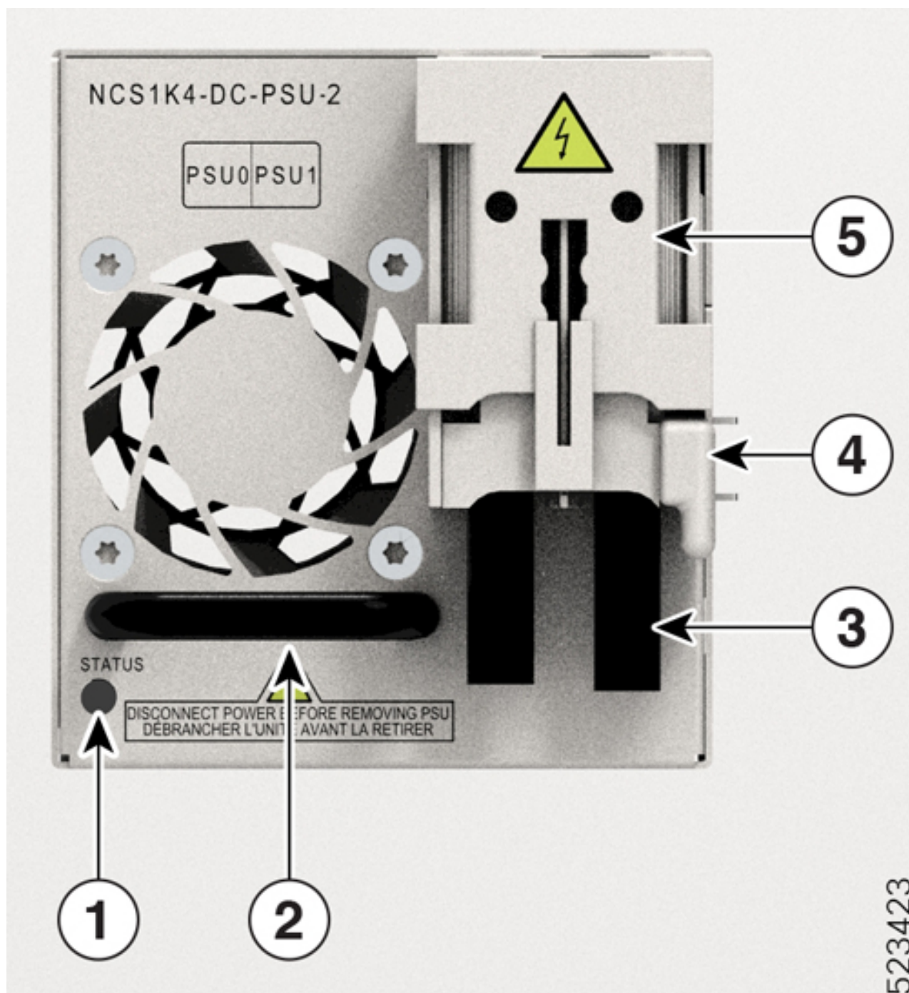
Figure 15: NCS1K4-DC-PSU-2 with 180-degree Power Lug Cable Connection
