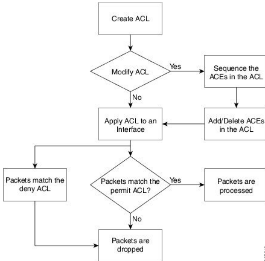
Figure 1: ACL Workflow
