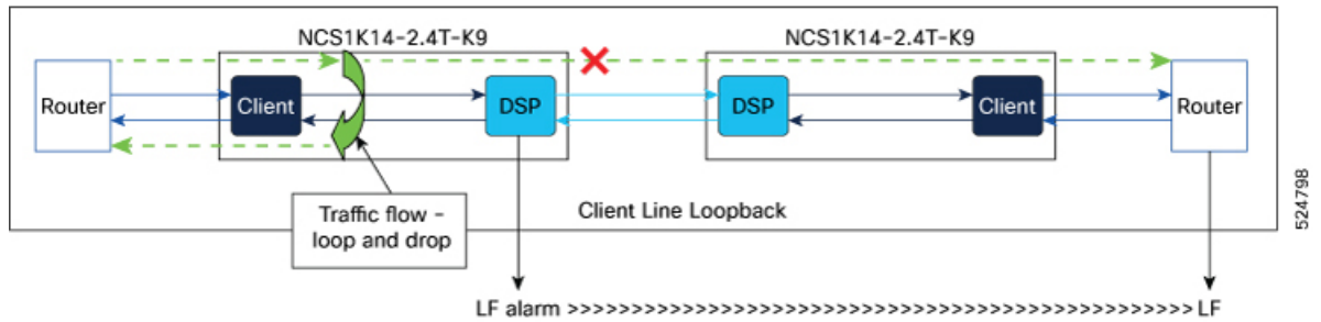
Figure 4: Line loop-and-drop
