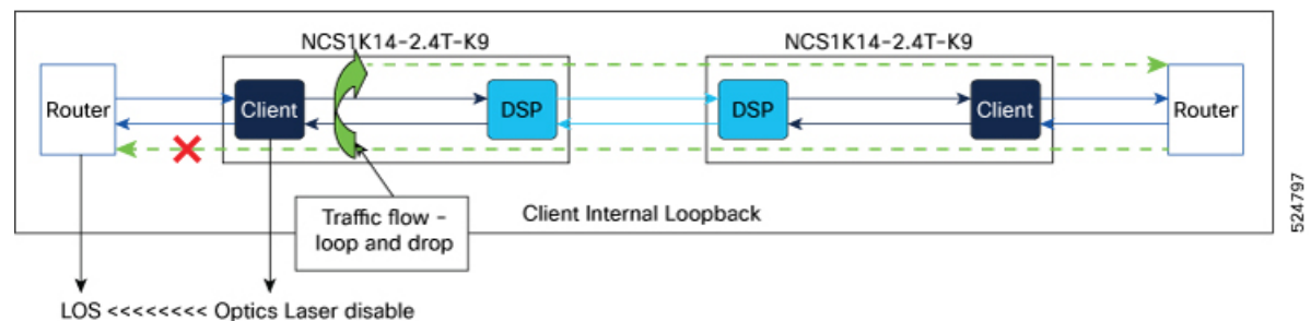
Figure 3: Internal loop-and-drop
