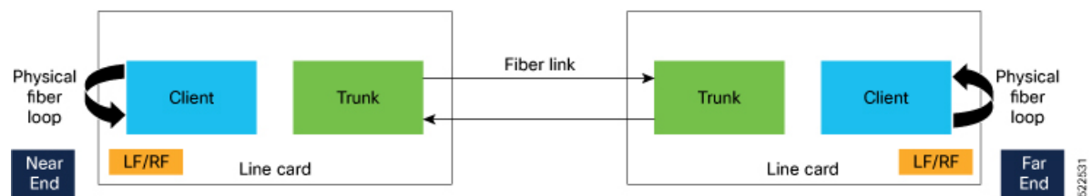
Figure 7: Topology for Link Verification
