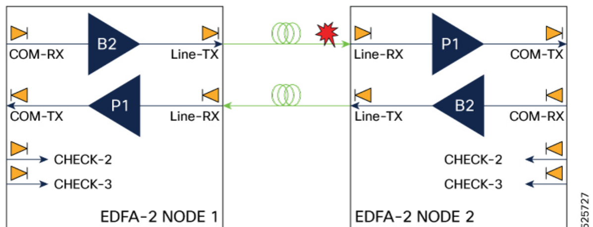
Figure 16: BST2 shutdown sequence
