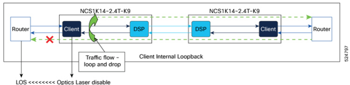
Figure 8: Internal loop-and-drop
