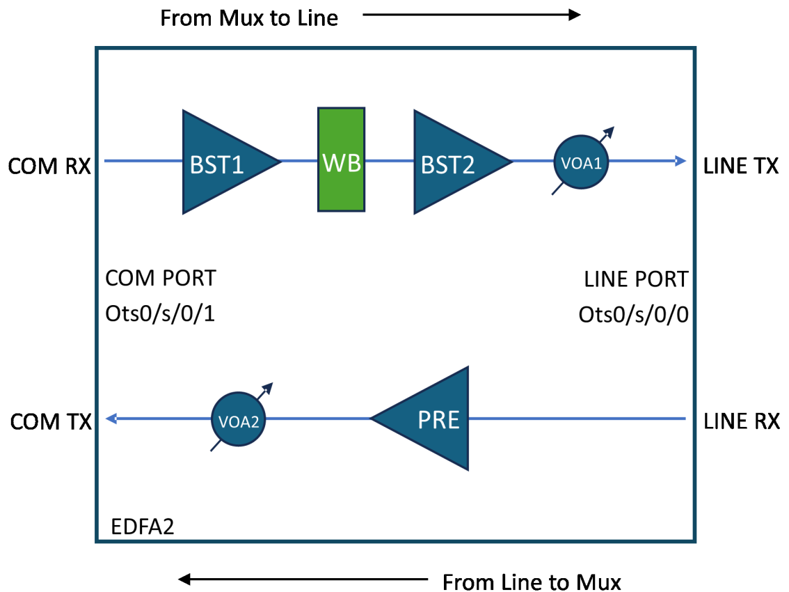
Figure 21: NCS1K14-EDFA2 line card optical layout
