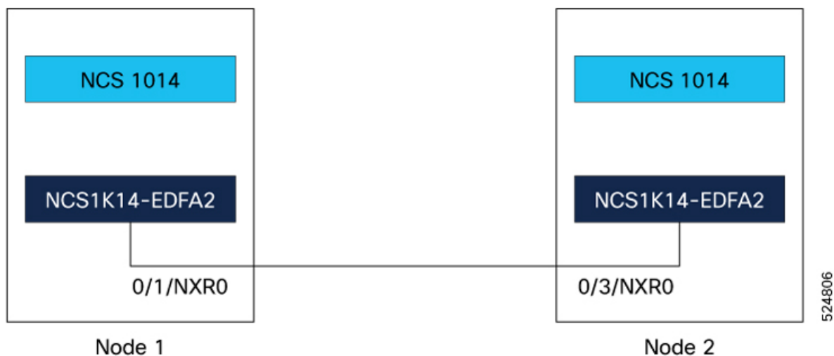
Figure 23: Sample two node topology
