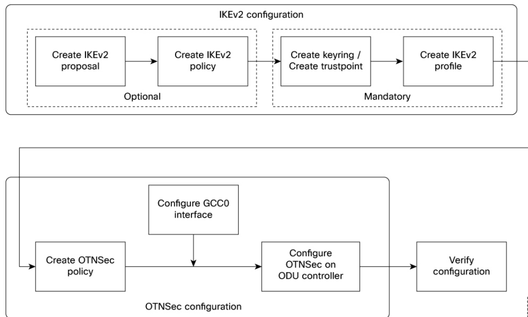
Figure 13: OTNSec configuration workflow
