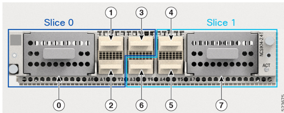
Figure 5: 2.4TX Line Card Slices and Ports
