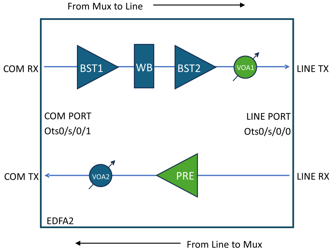
Figure 22: NCS1K14-EDFA2 line card optical layout
