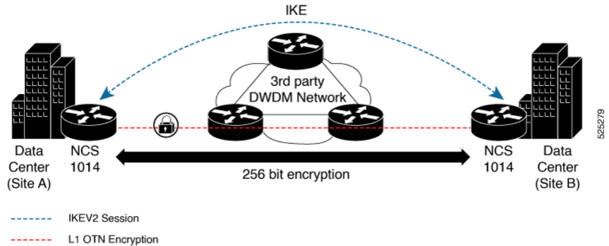
Figure 10: OTNSec site-to-site example and components
