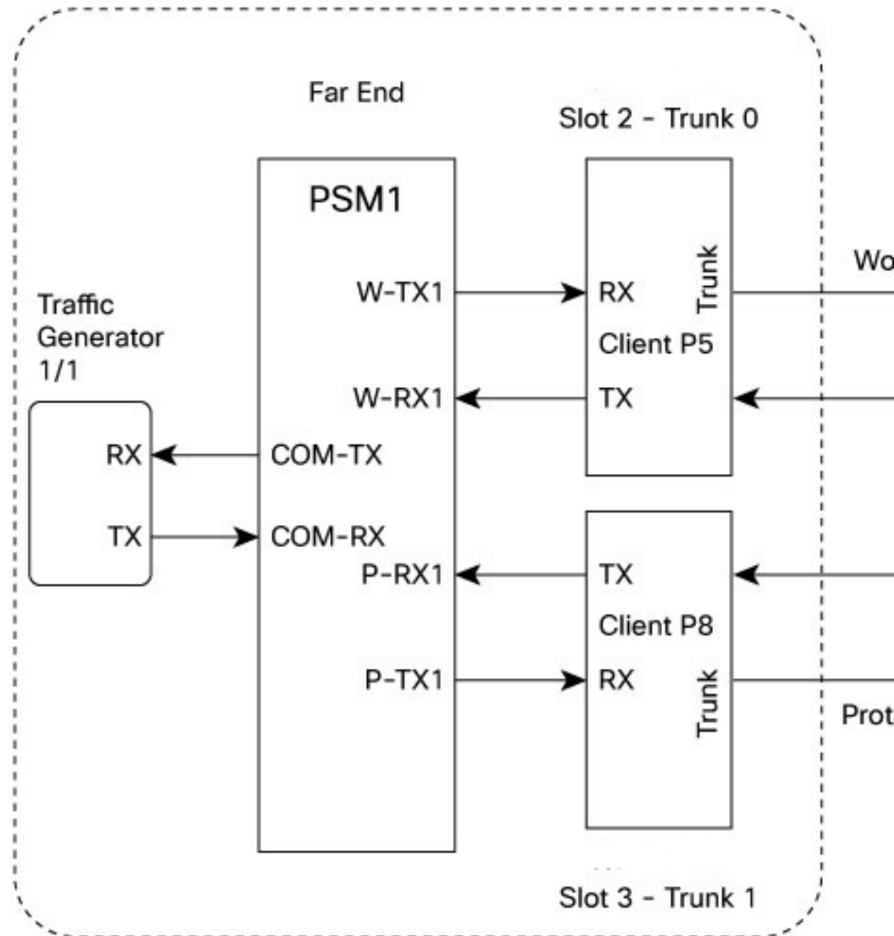
Figure 6: Reference Topology for Protection Switching
