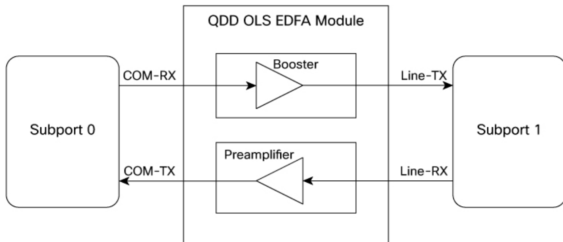
Figure 3: Functional description of QDD OLS
