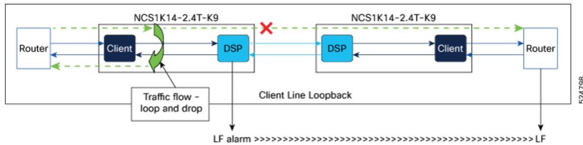
Figure 4: Line loop-and-drop
