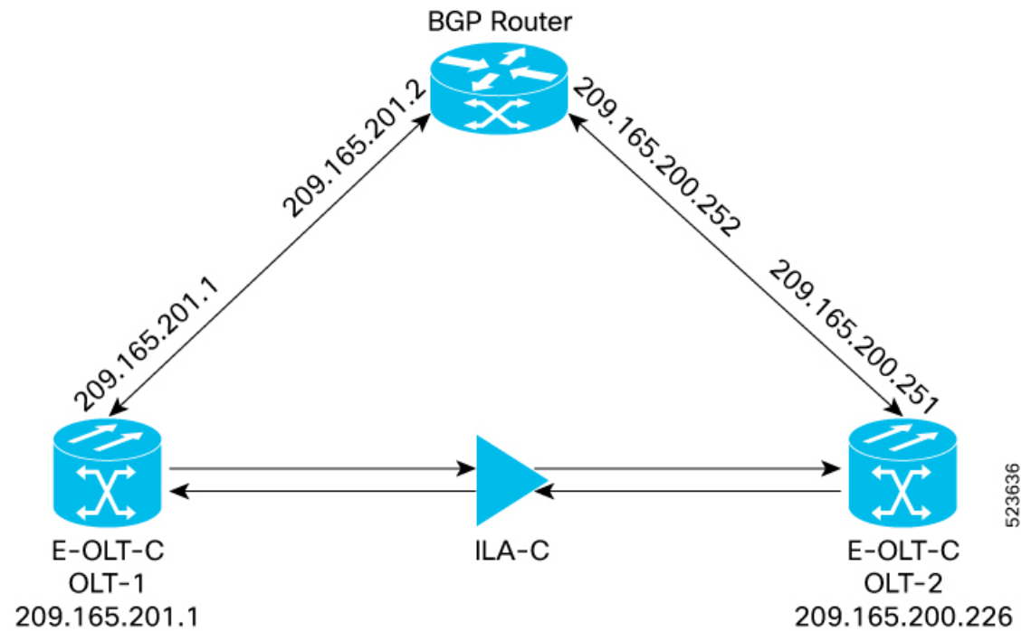
Figure 1: BGP Topology
