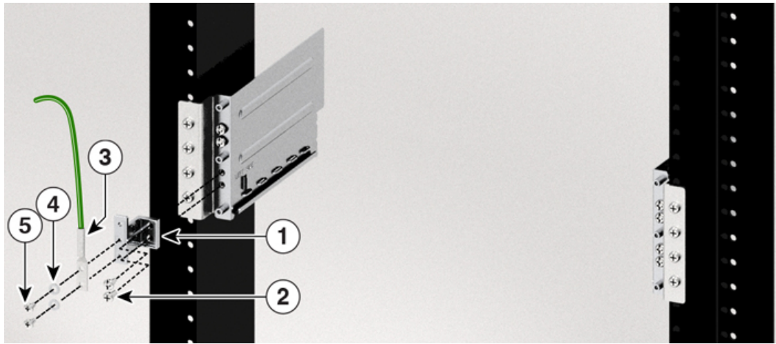
Figure 7: Fixing Ground Lug on the Ground Adapter - ETSI Rack
