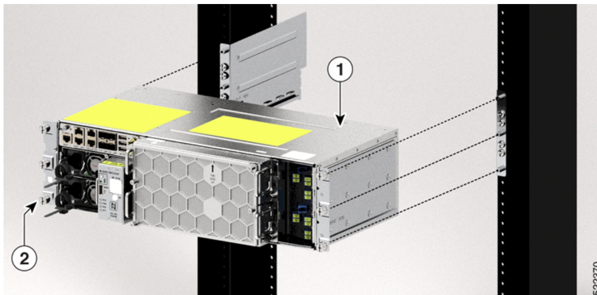
Figure 10: Mounting the Chassis on the Rack
