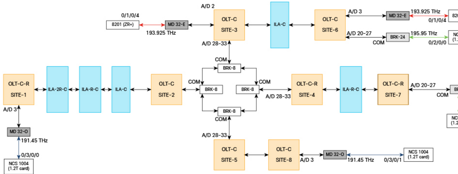
Figure 1: Multi-degree Topology
