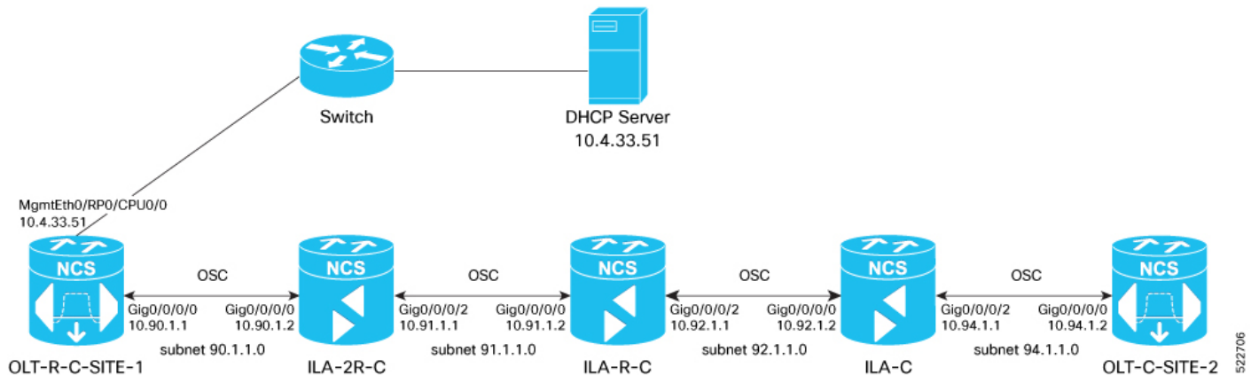
Figure 2: NetworkTopology Diagram
