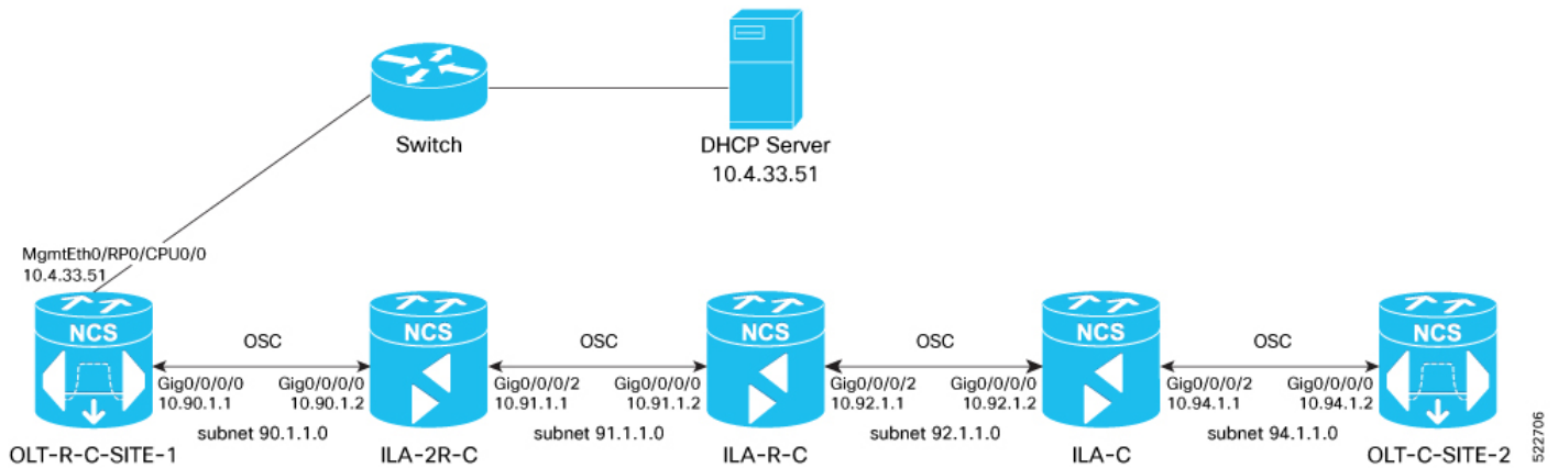
Figure 4: NetworkTopology Diagram
