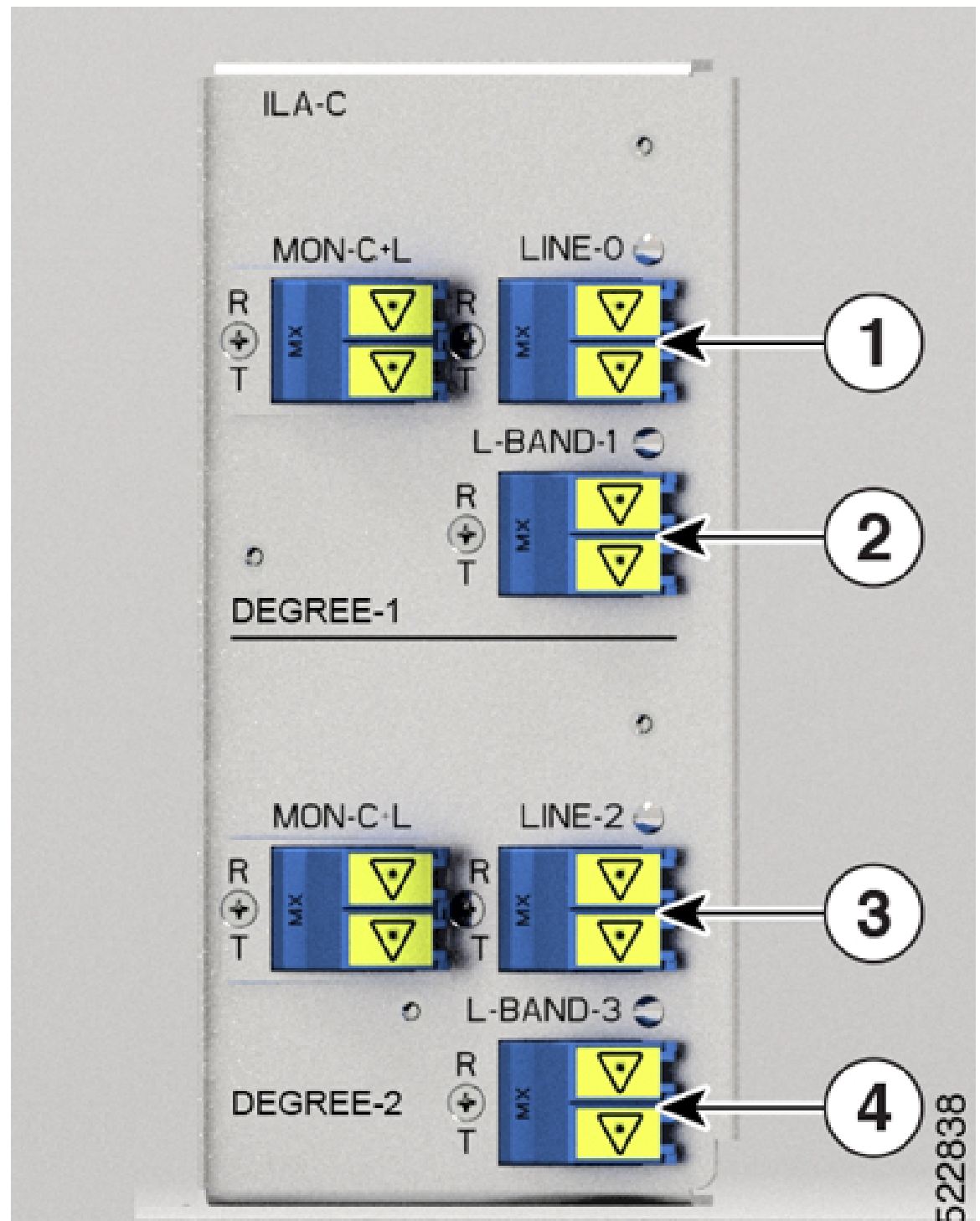
Figure 1: NCS1K-ILA-C front view
