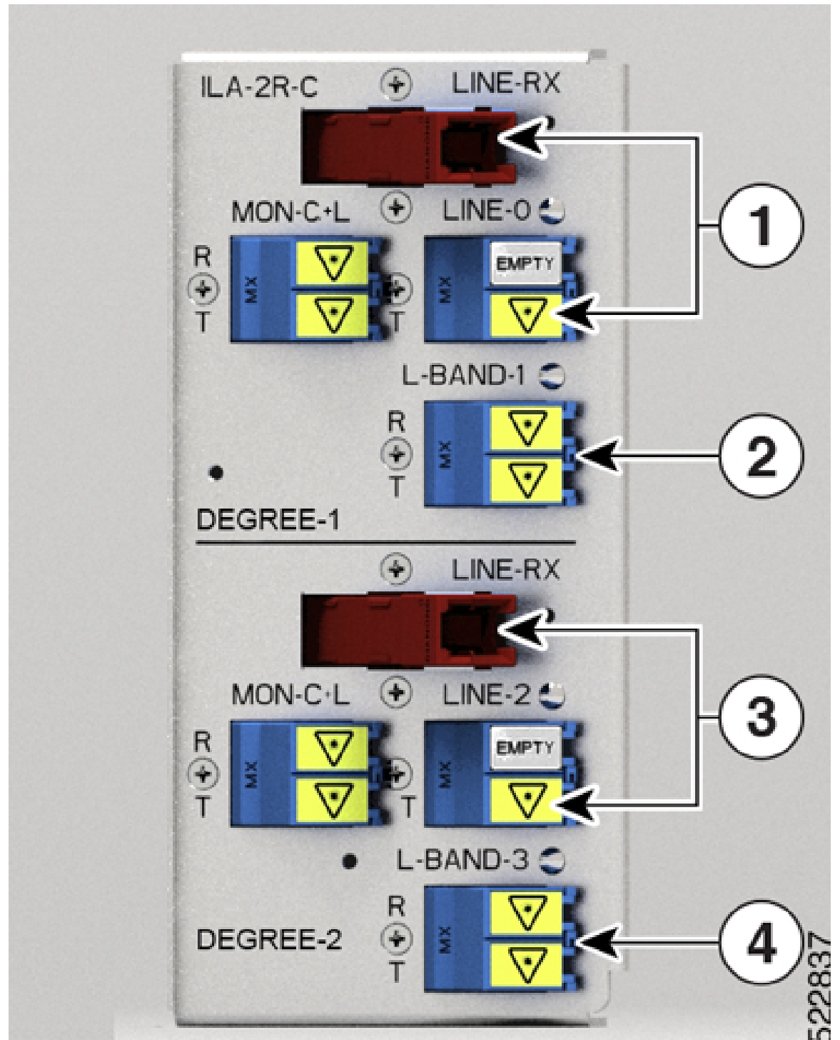
Figure 3: NCS1K-ILA-2R-C front view
