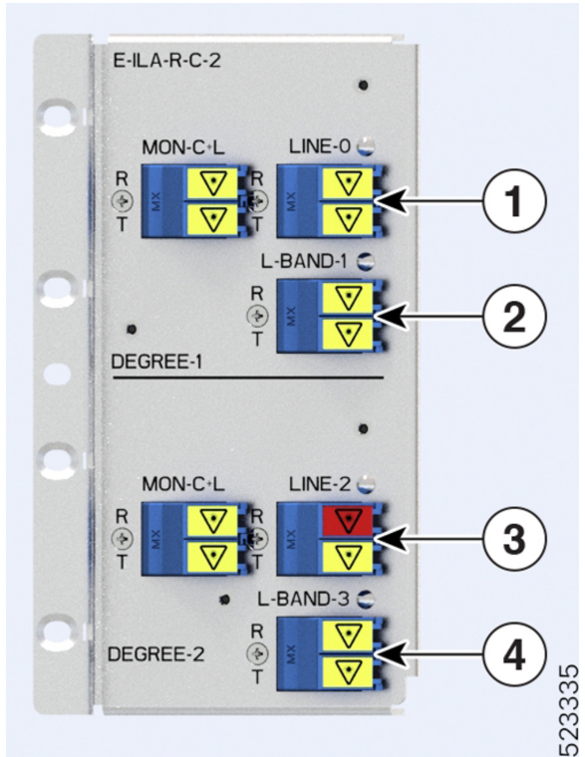
Figure 7: NCS1K-E-ILA-R-C-2 front view
