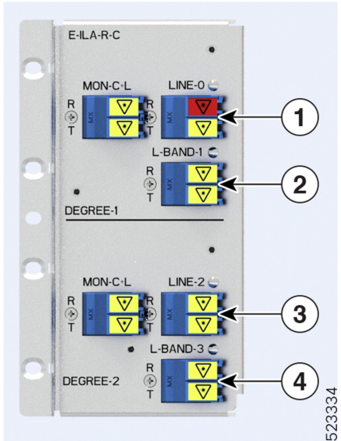
Figure 5: NCS1K-E-ILA-R-C front view
