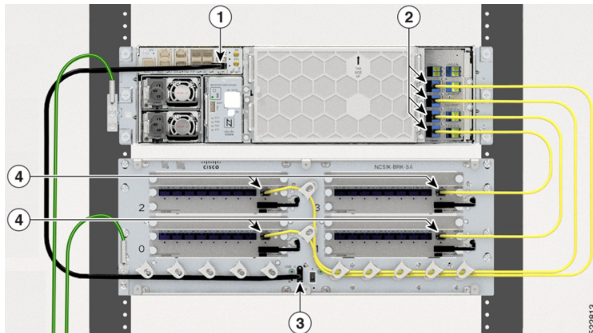
Figure 3: NCS 1010 and NCS1K-BRK-8 Connection
