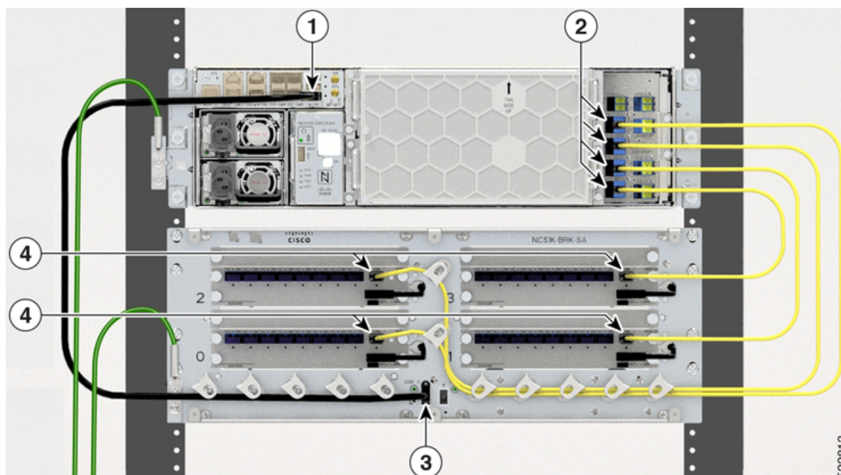
Figure 3: NCS 1010 and NCS1K-BRK-8 Connection
