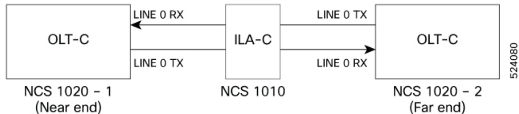
Figure 1: Sample two node topology of NCS 1020 nodes
