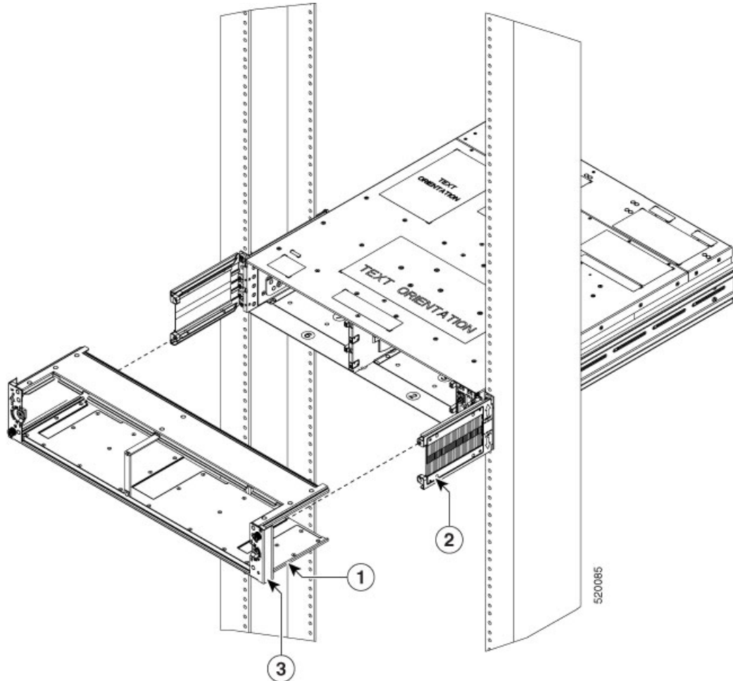
Figure 21: Installing the Air Filter Frame and Side Brackets
