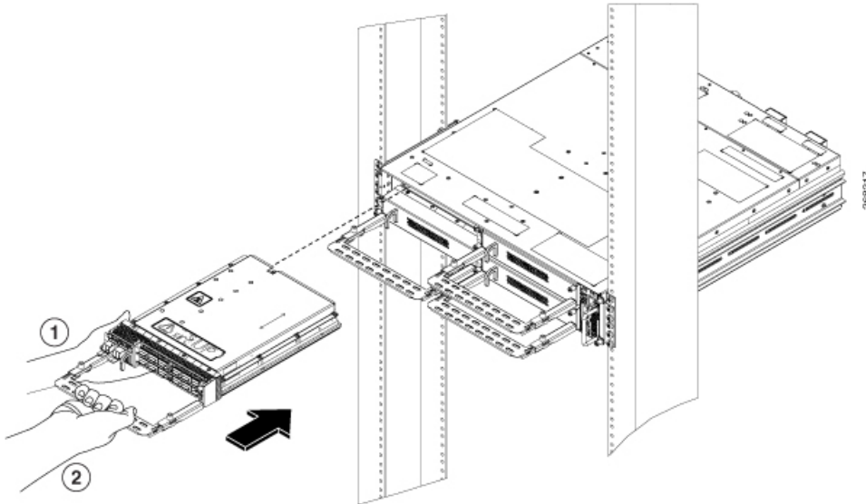
Figure 2: Installing the 1.2T, 1.2TL, and 2-QDD-C Line Cards
