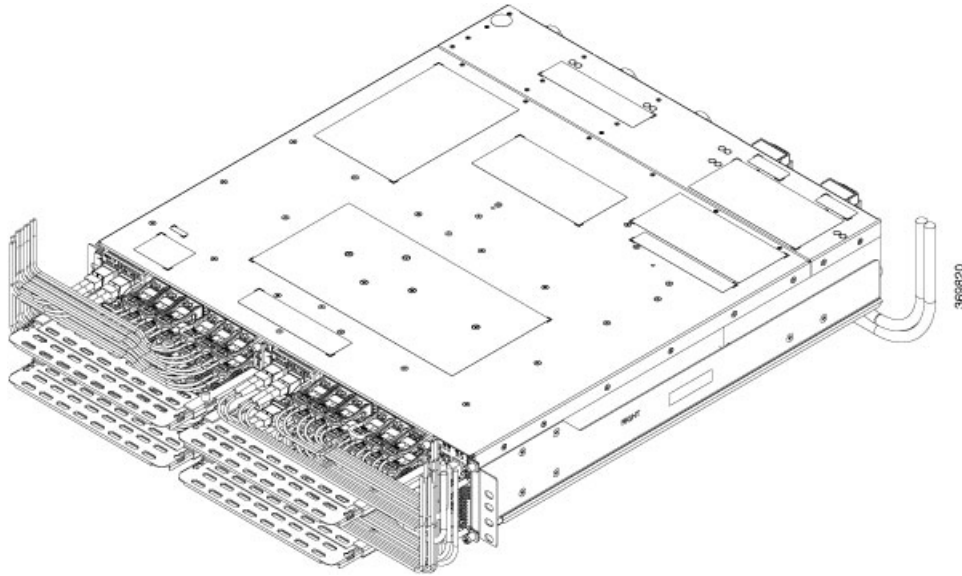
Figure 20: Fiber Management Bracket for the OTN-XP Line Card
