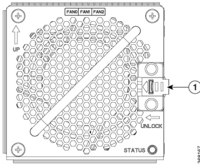
Figure 11: Spring-loaded Lever in Released Condition
