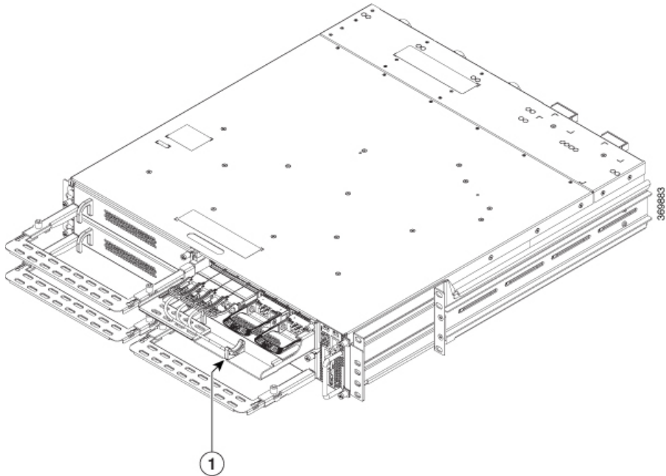
Figure 20: Fiber Management Bracket for the OTN-XP Line Card
