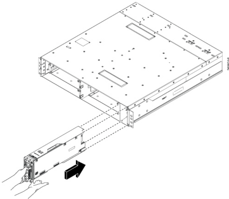
Figure 9: Installing the Controller Unit
