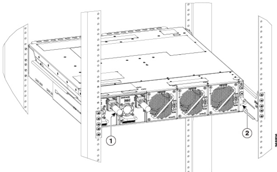
Figure 8: Connecting Straight Power Cable
