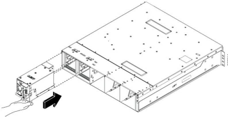
Figure 3: Installing a PSU
