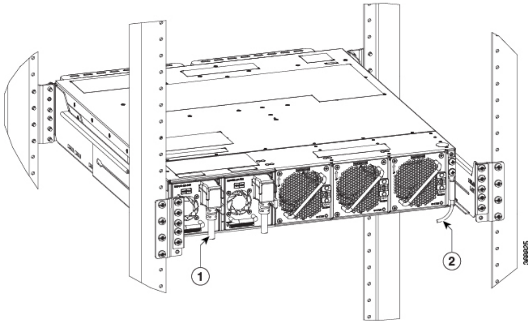
Figure 7: Connecting 90-degree Power Cable
