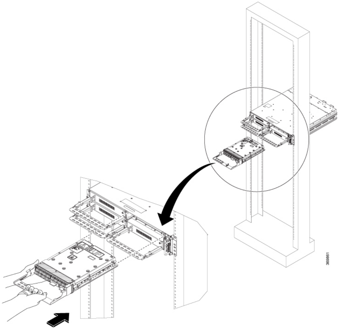
Figure 1: Installing the OTN-XP Line Card
