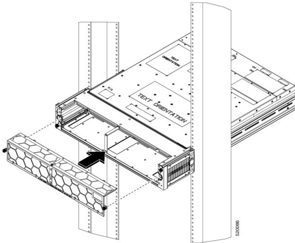
Figure 22: Installing the Air Filter
