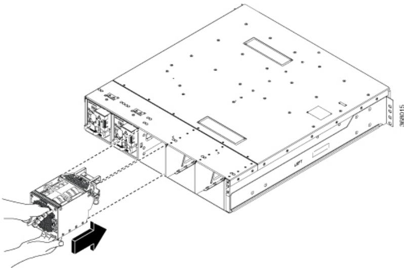
Figure 10: Inserting a Fan unit
