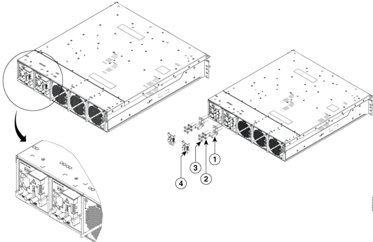
Figure 5: Connecting DC Power
