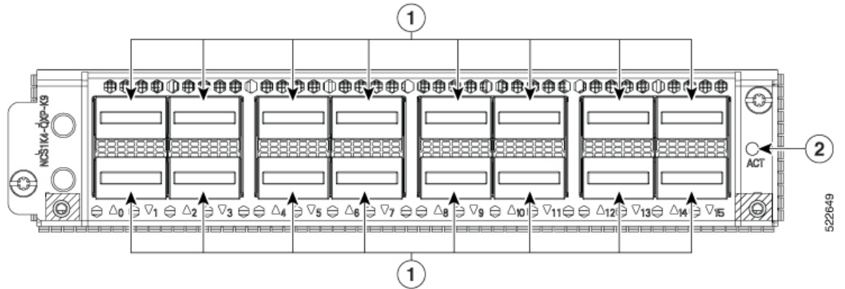
Figure 5: Front View of the QXP-K9 Line Card
