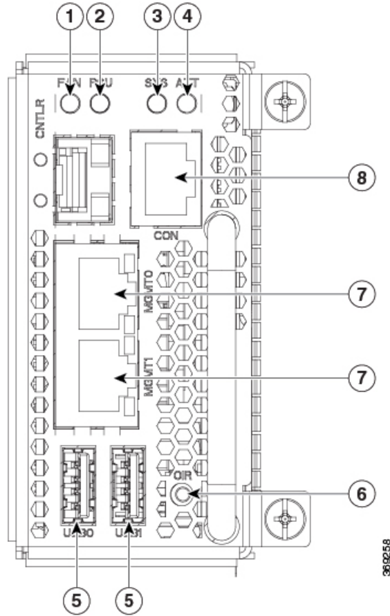
Figure 6: Front View of the Controller
