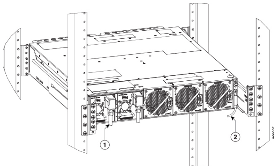
Figure 8: Connecting 90-degree Power Cable
