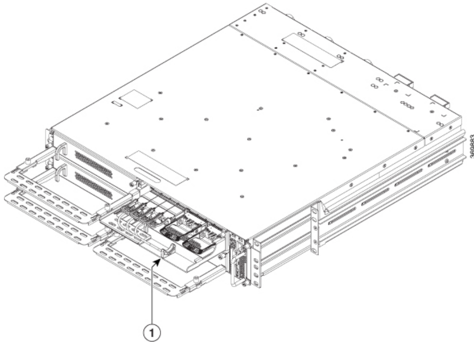
Figure 21: Fiber Management Bracket for the OTN-XP Line Card
