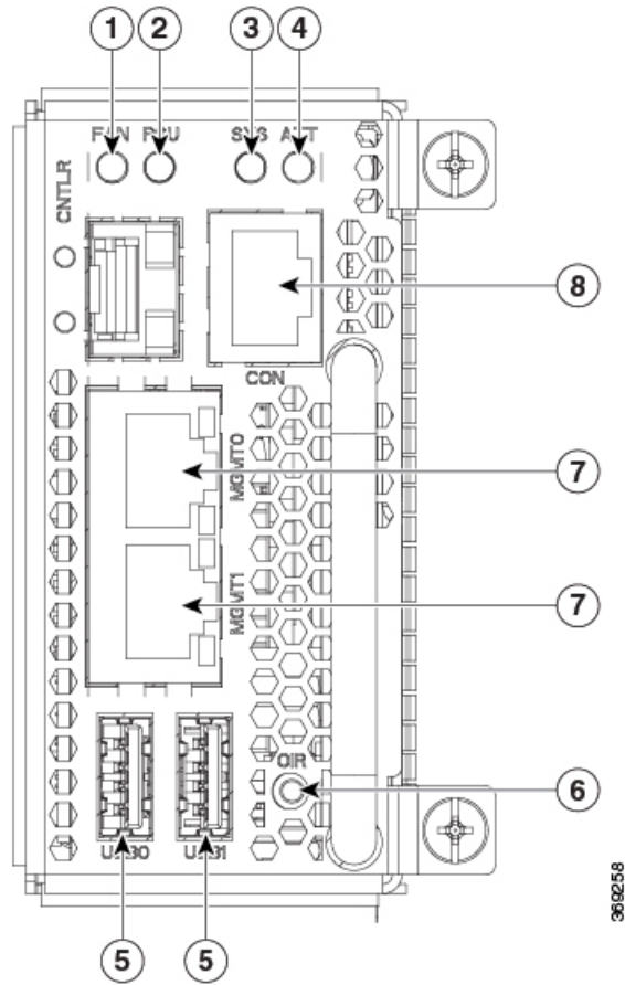
Figure 2: Front View of the Controller
