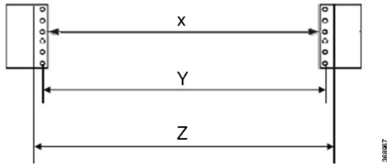
Figure 4: Rack Specification
