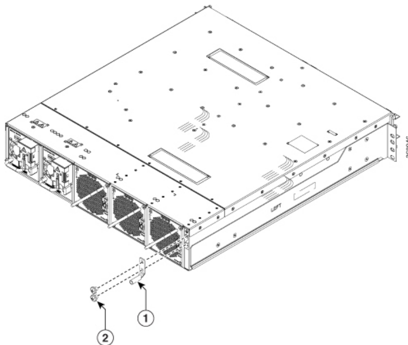
Figure 20: NCS 1004 Ground Lug
