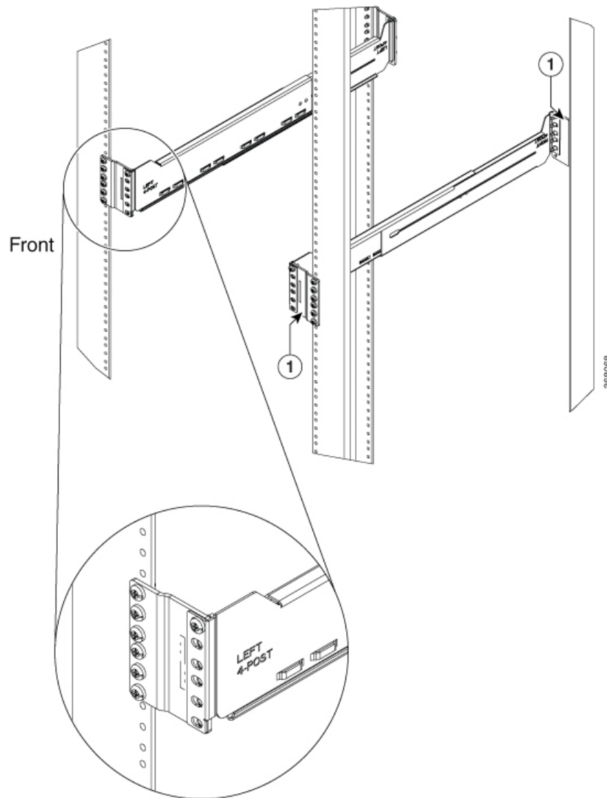
Figure 17: Four Post Slider Integration - ETSI Rack
