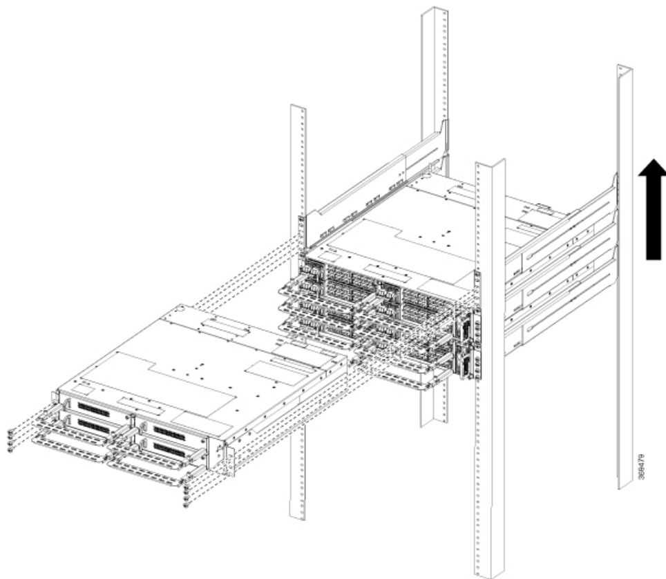
Figure 18: Stacking the NCS 1004
