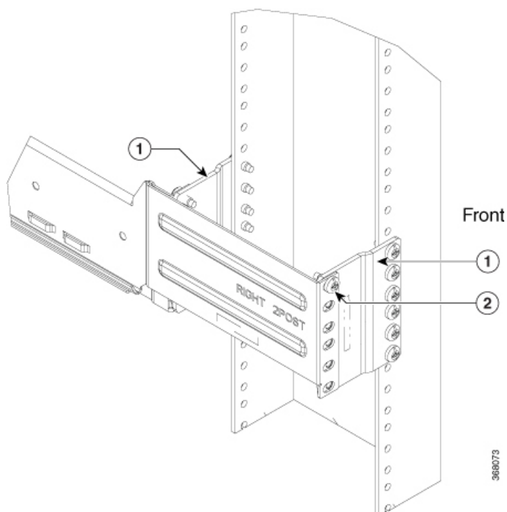
Figure 10: Two Post Slider Integration - 23" Rack
