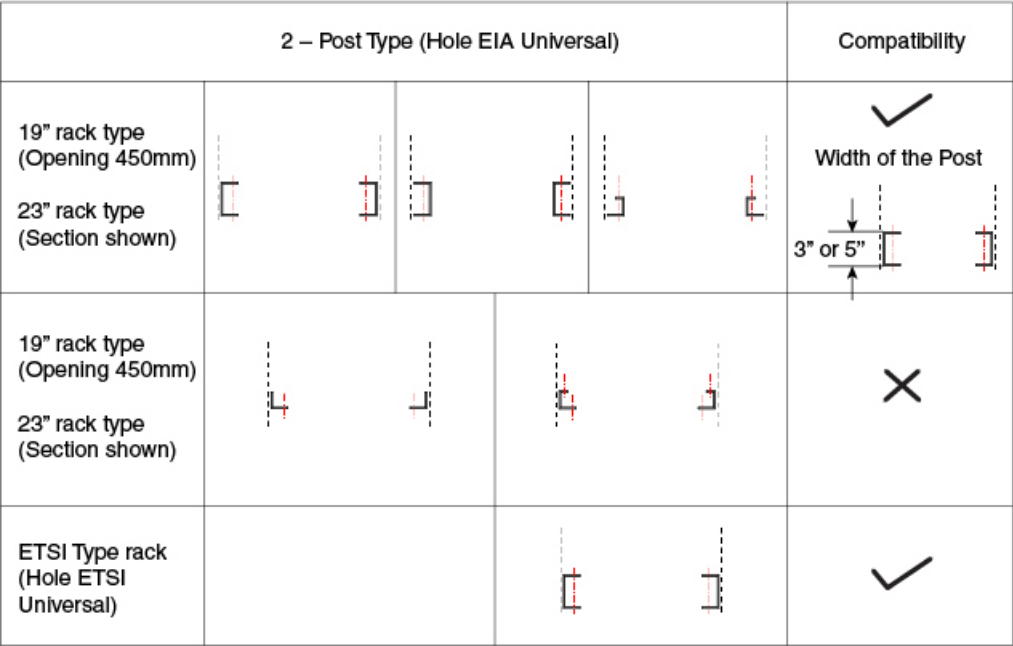
Figure 3: Two Post Rack Type
