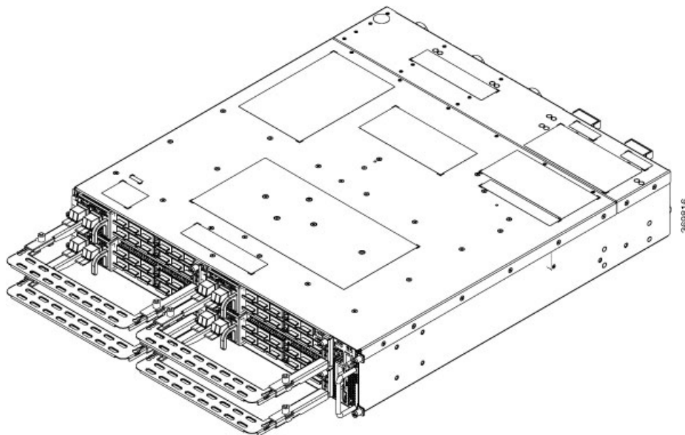
Figure 6: Filler Cards fitted with Fiber Management Bracket
