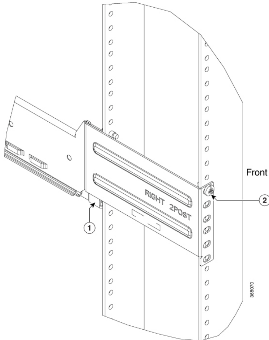
Figure 9: Two Post Slider Integration - 19" Rack
