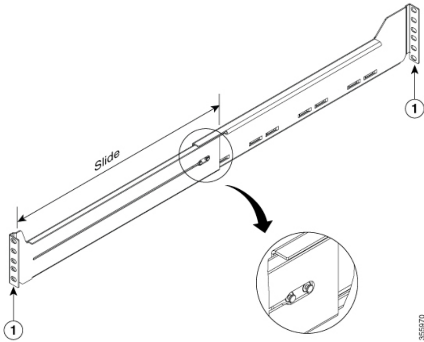
Figure 16: Four Post Slider Identification
