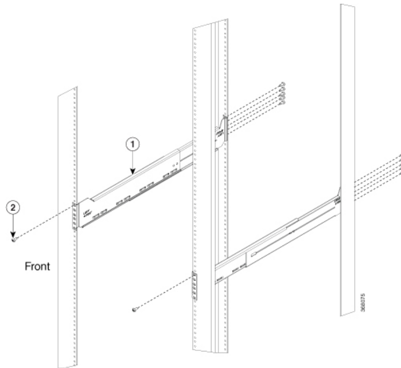
Figure 12: Four Post Slider Integration - 19" Rack
