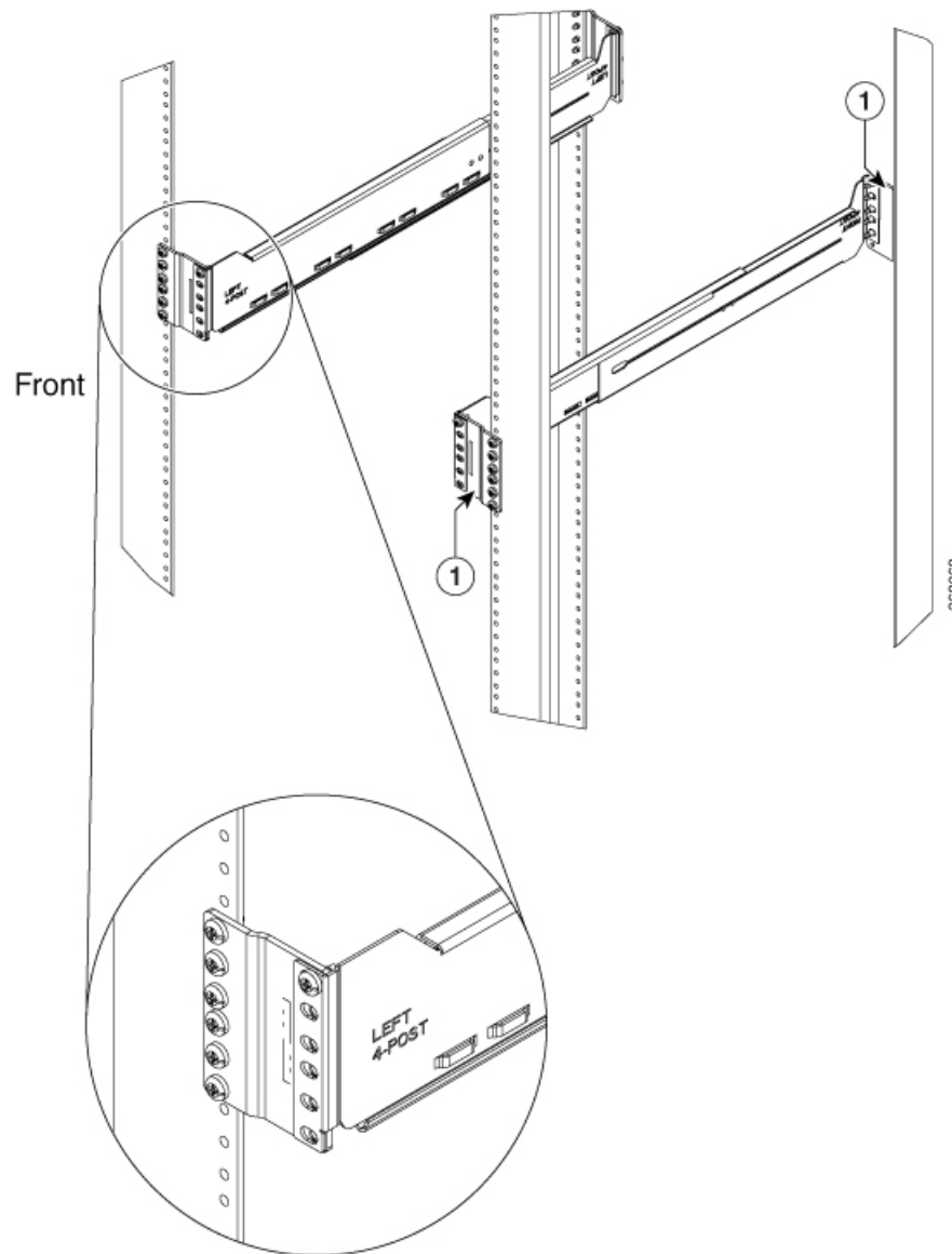
Figure 13: Four Post Slider Integration - 23" Rack
