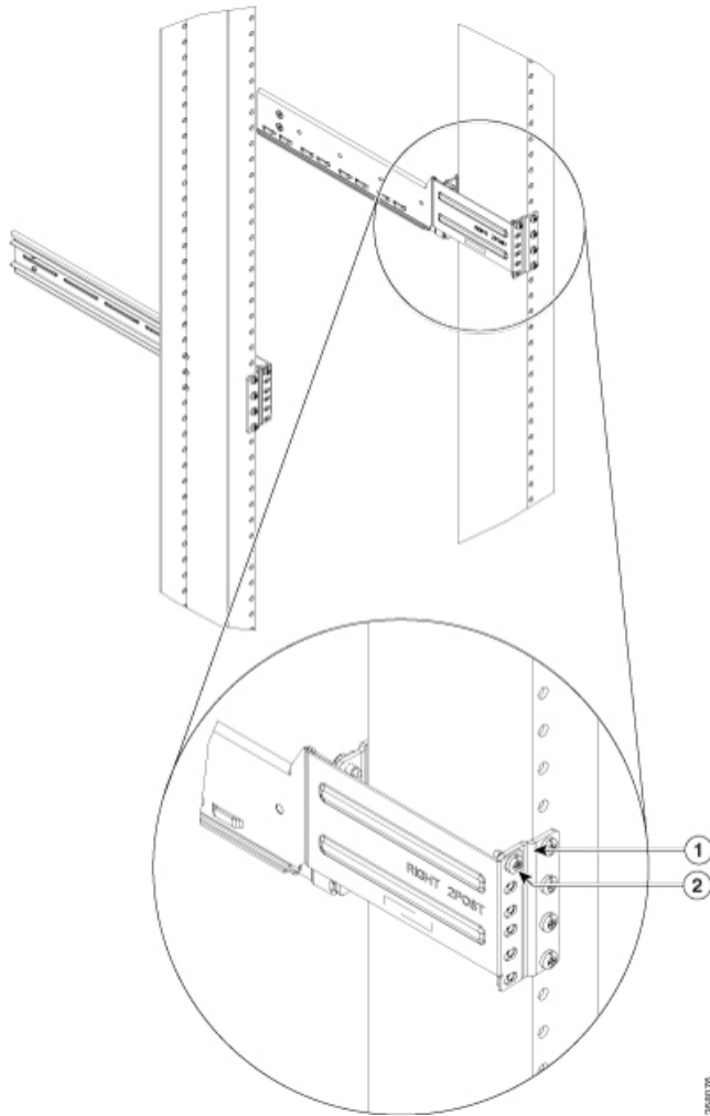
Figure 15: Two Post Slider Integration - ETSI Rack
