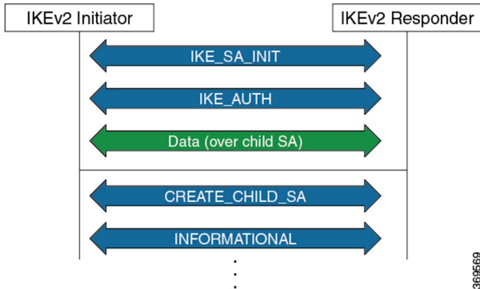
Figure 2: IKEv2 Exchanges
