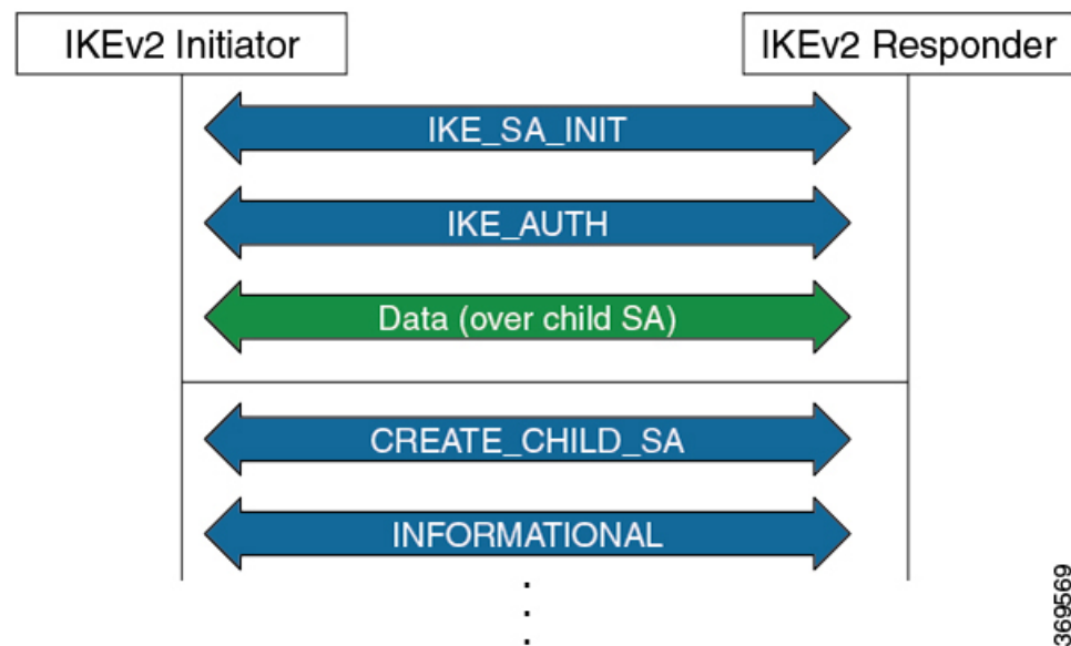
Figure 6: IKEv2 Exchanges
