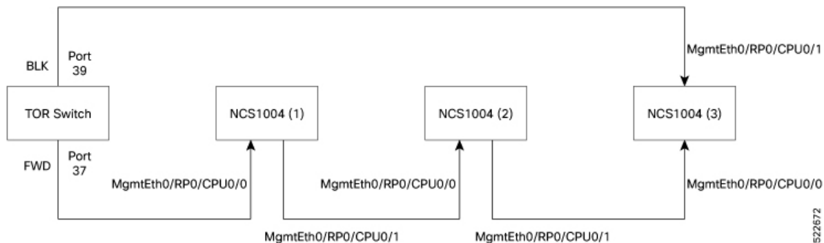
Figure 2: Daisy Chain Topology
