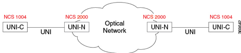
Figure 7: GMPLS UNI Reference Model
