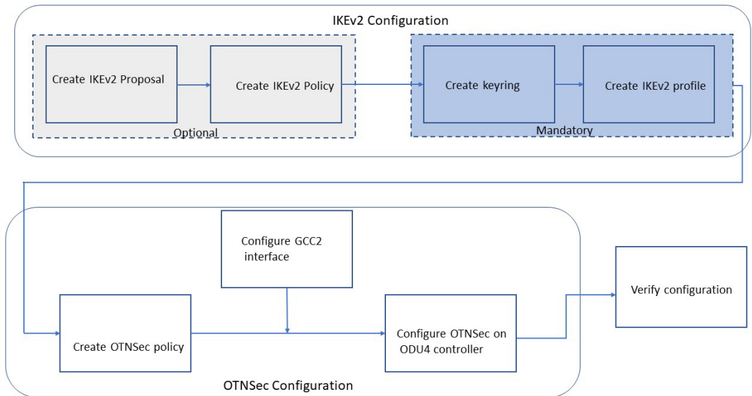
Figure 5: L1 Encryption Workflow
