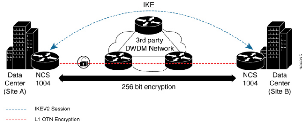
Figure 3: OTNSec Site-to-Site Example and Components
