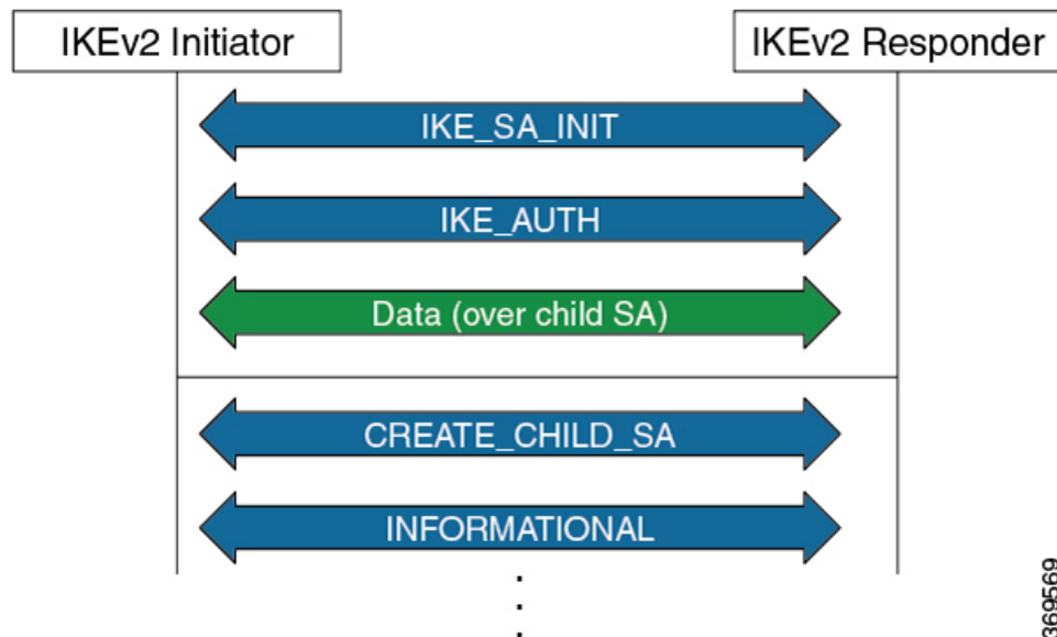
Figure 4: IKEv2 Exchanges
