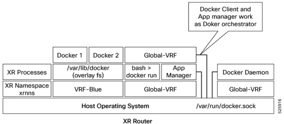
Figure 1: Docker on IOS XR
