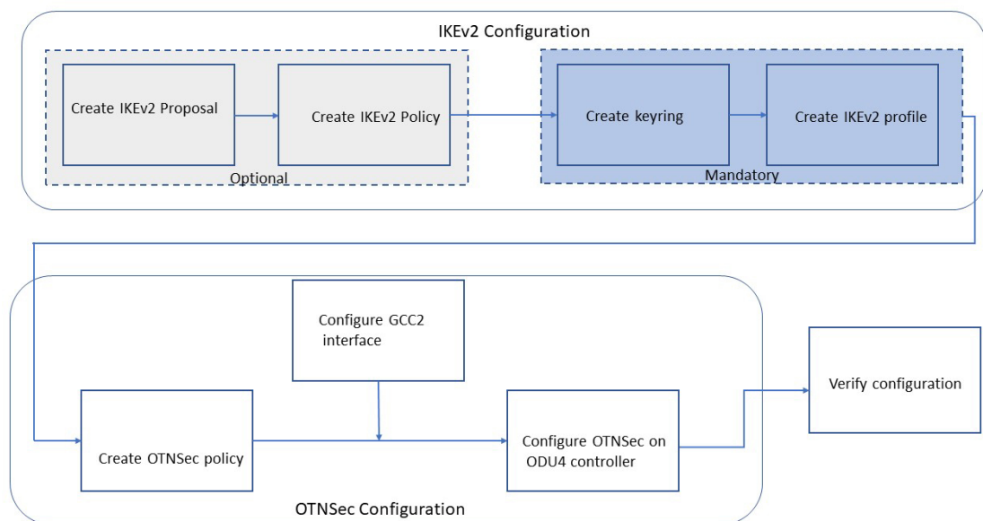
Figure 5: L1 Encryption Workflow
