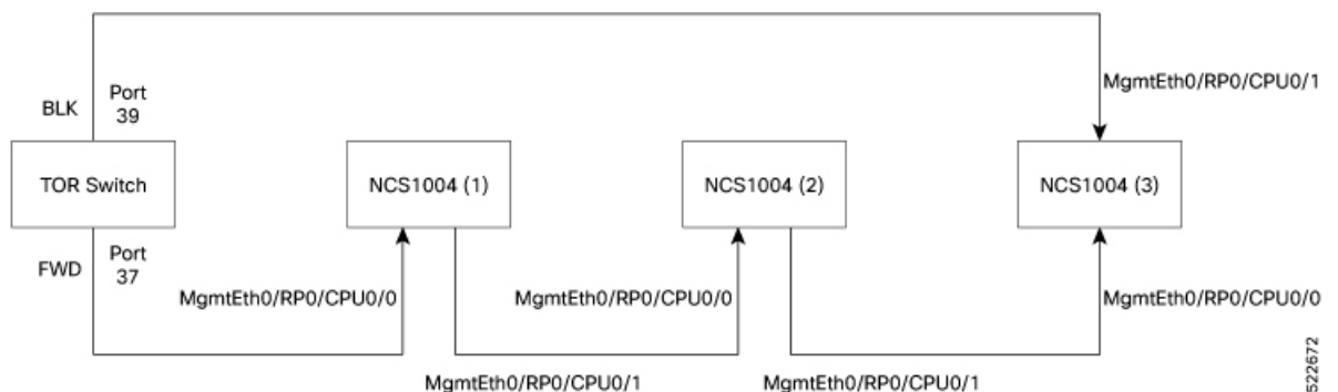
Figure 2: Daisy Chain Topology
