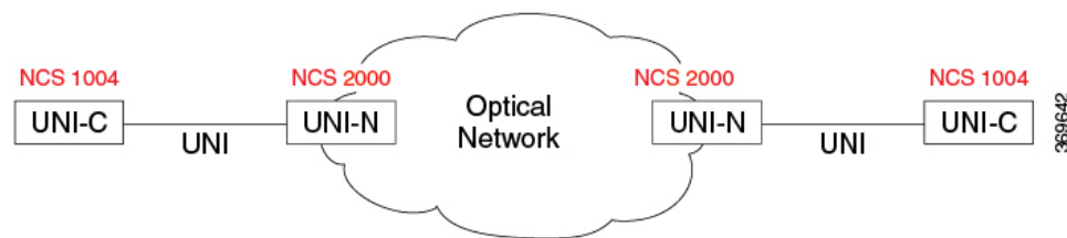
Figure 1: GMPLS UNI reference model
