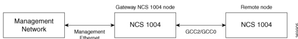
Figure 13: Remote Node Management in Linear Topology
