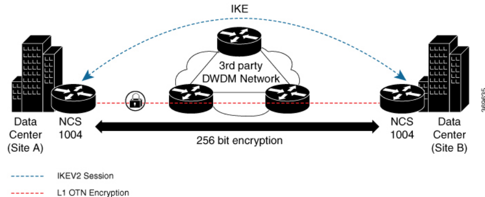
Figure 5: OTNSec Site-to-Site Example and Components
