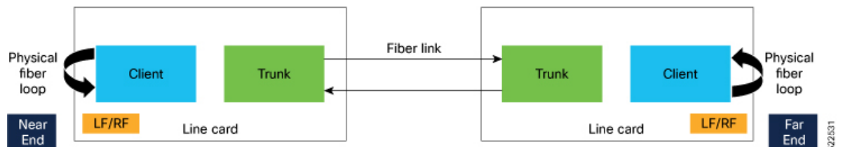
Figure 2: Topology for Link Verification
