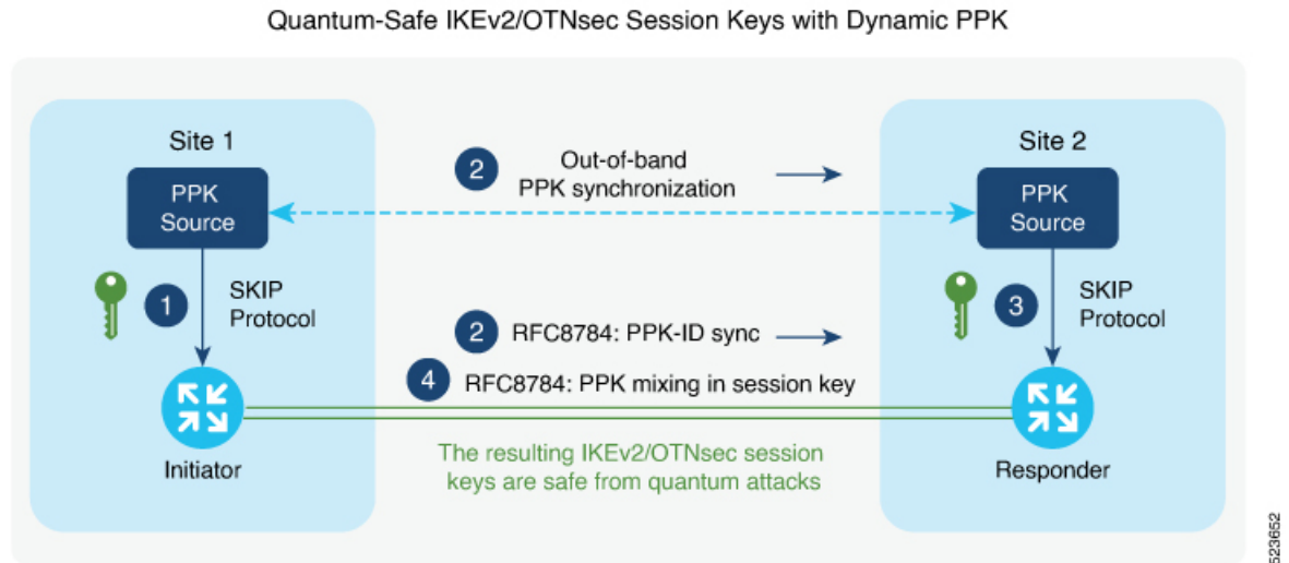
Figure 10: Quantum-Safe IKEv2 and OTNsec Session Keys with Dynamic PPK
