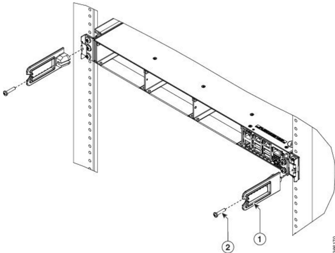
Figure 23: Cable Guide
