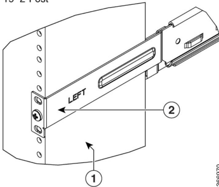
Figure 19: Mating for the Two Post 19" Rack
