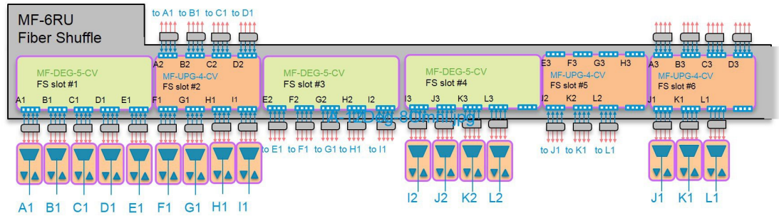
Figure 8: Add/Drop Stage
