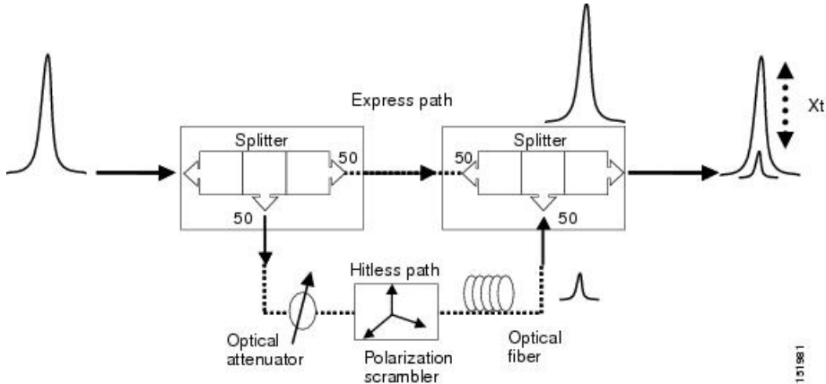
Figure 5: Block Diagram for Crosstalk Measure
