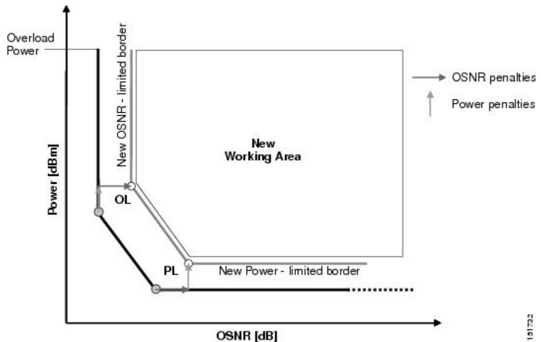
Figure 2: Interface Margin Application
