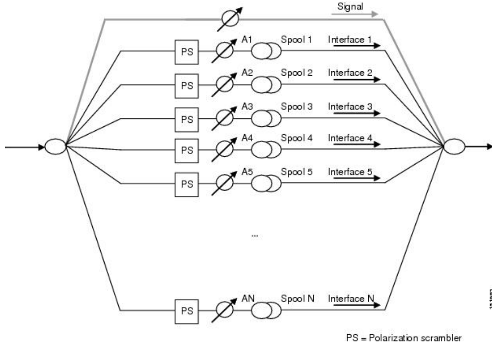
Figure 6: Generation Block for Gaussian Cross-Talk Measurement
