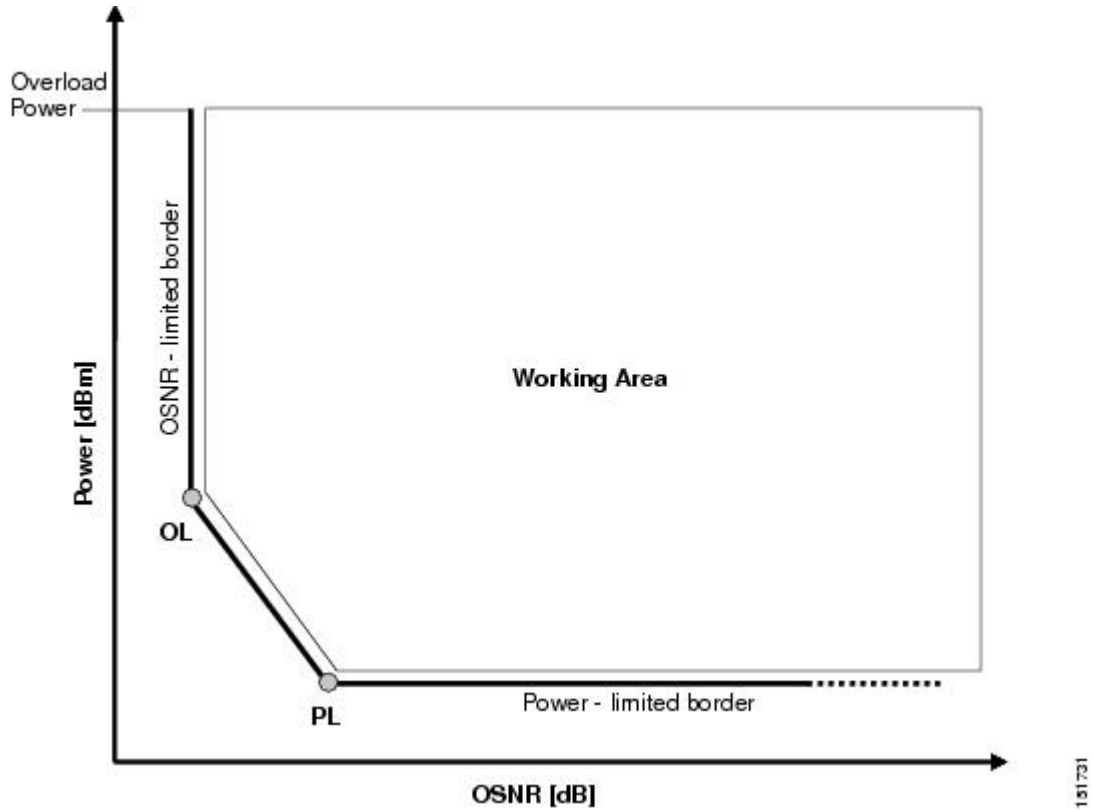
Figure 1: Interface Operative Area
