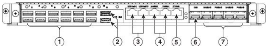
Figure 17: Connectors on the NCS 2015 ECU Faceplate
