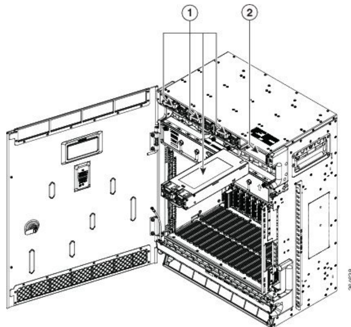
Figure 20: Installing the DC power module
