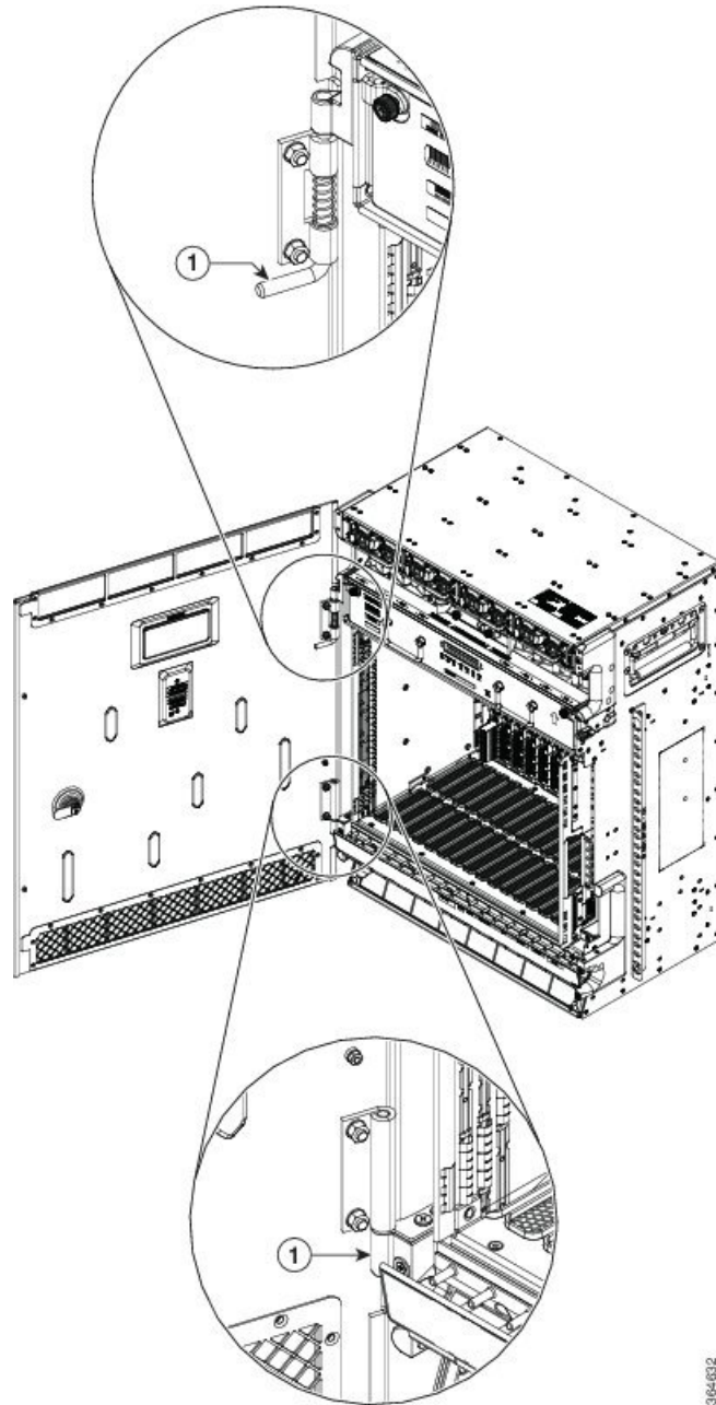
Figure 7: Hinge Pins
