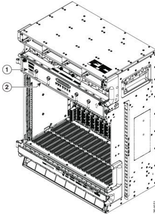
Figure 23: Fan Tray Assembly Installed in NCS 2015 DC Shelf
