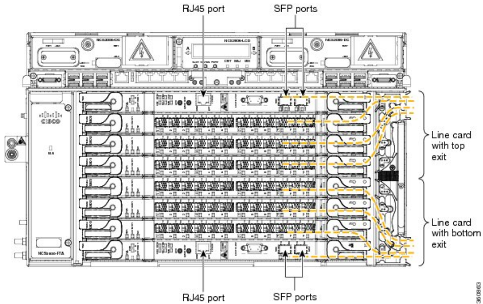
Figure 6: Cable Routing
