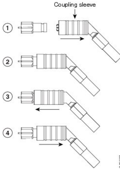
Figure 13: Sequence to Attach the Connectors
