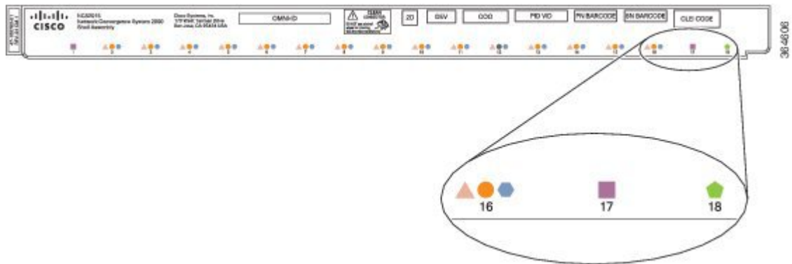
Figure 3: Slot Symbols
