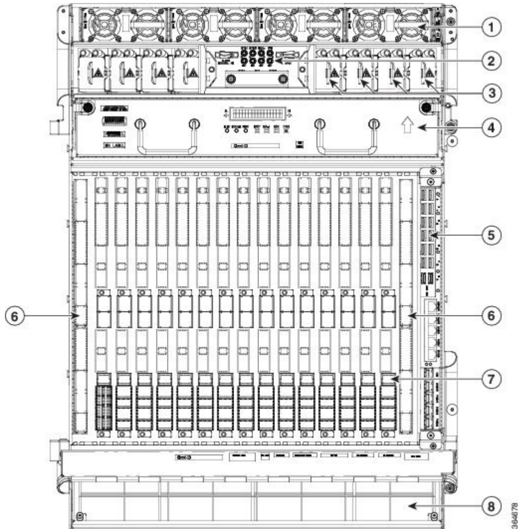
Figure 7: Front View of the NCS 2015 DC Chassis
