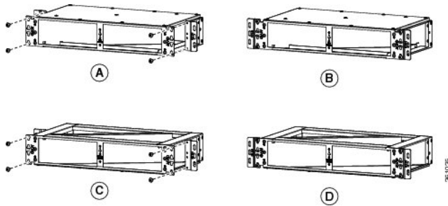
Figure 17: Installing the adapter plates on the horizontal air plenum
