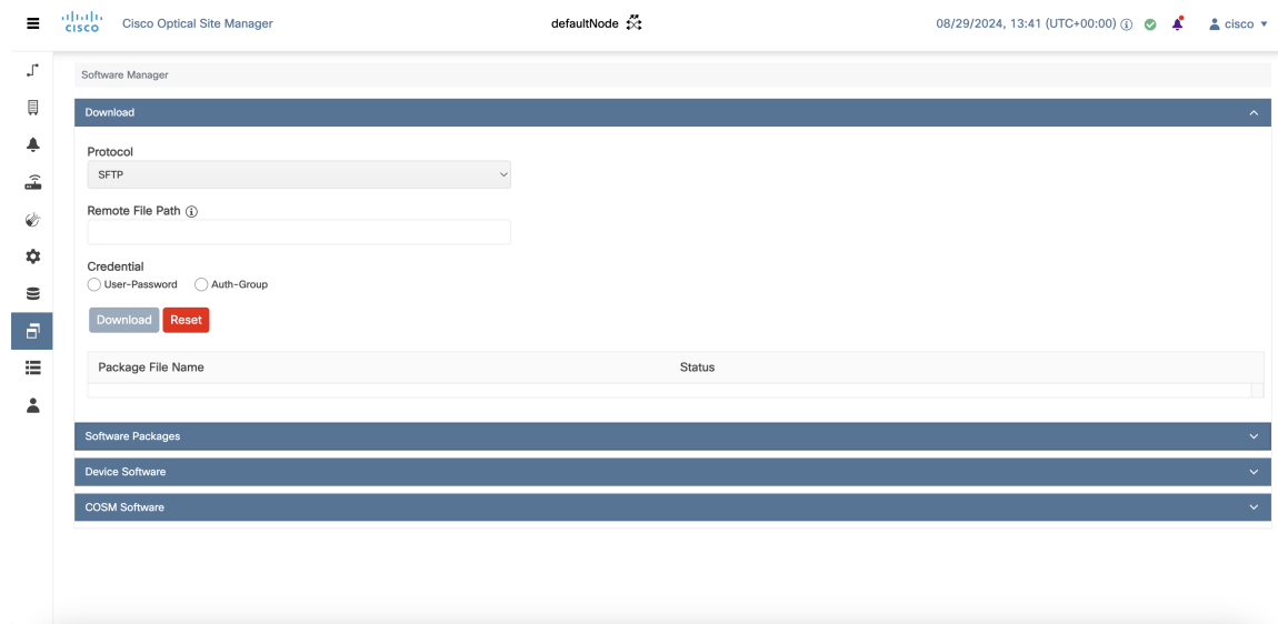
Figure 1: Software Upgrade
