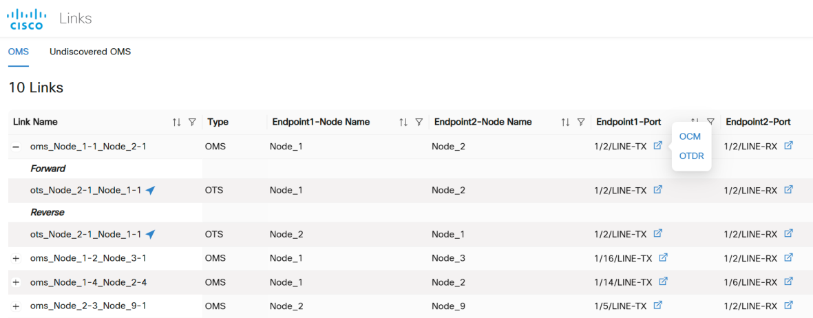
Figure 85: Links App
