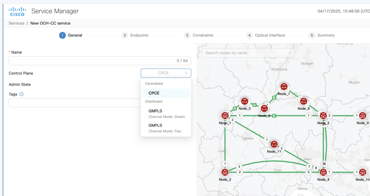
Figure 28: Service Manager
