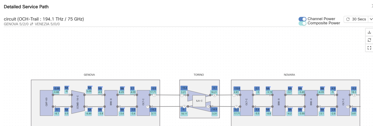
Figure 56: Live PM Channel and Composite Power Values
