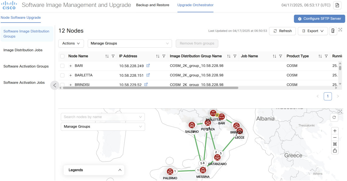
Figure 67: Upgrade Orchestrator
