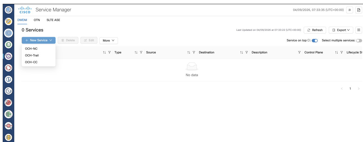
Figure 33: Service Manager
