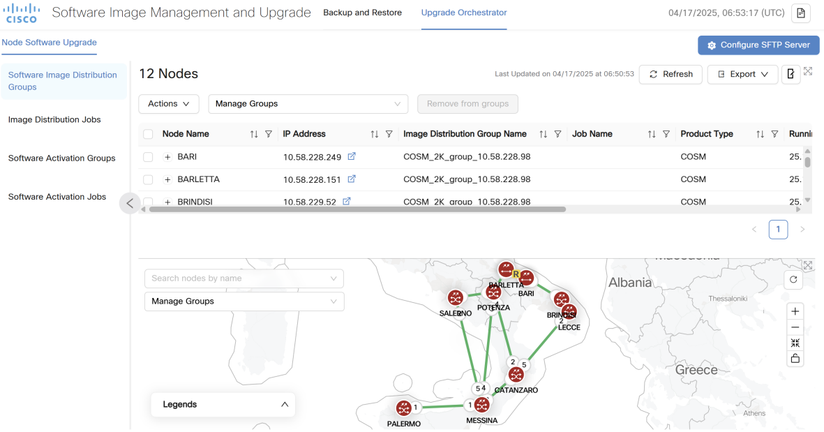
Figure 68: Upgrade Orchestrator
