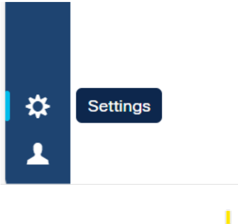
Figure 3: Settings Options
