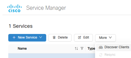
Figure 32: Service Manager
