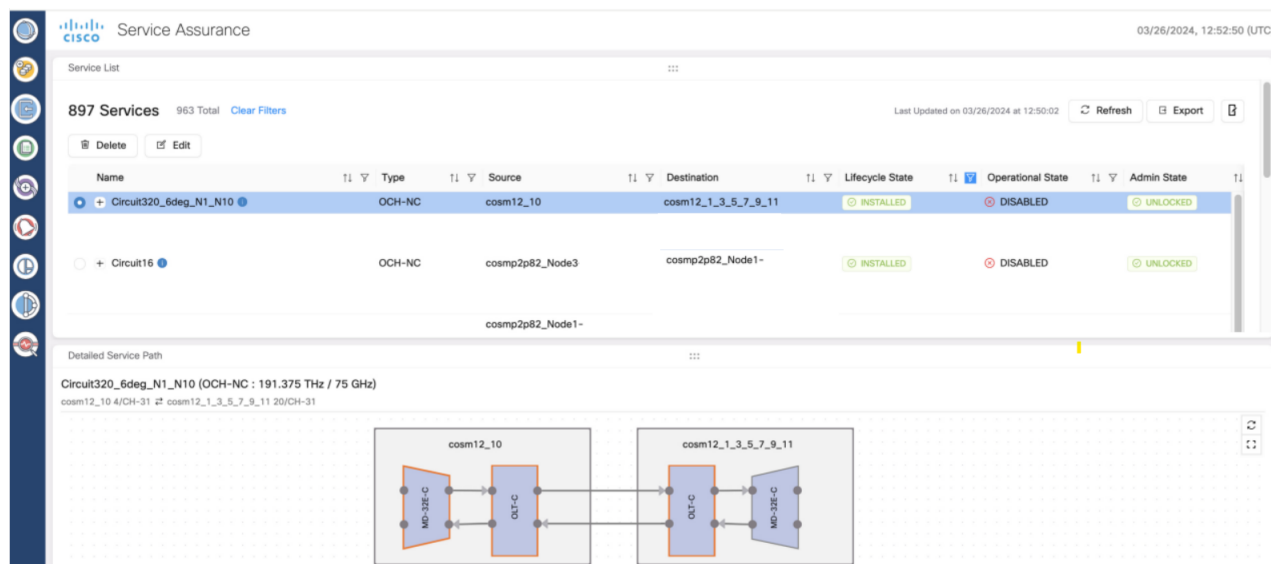
Figure 55: Service Assurance
