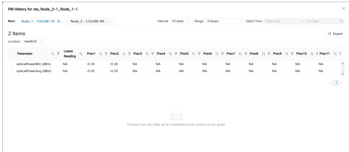
Figure 84: Links App
