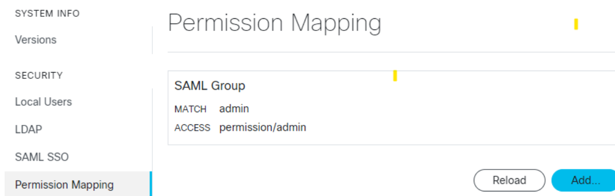
Figure 8: Permission Mapping
