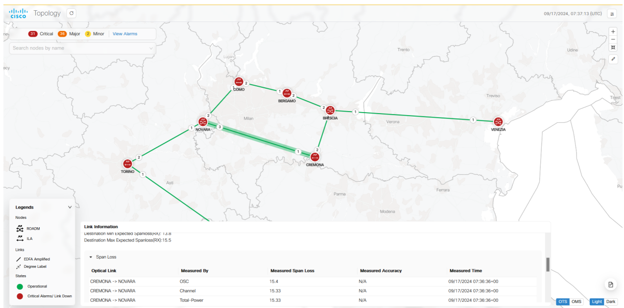
Figure 16: Tool Tip
