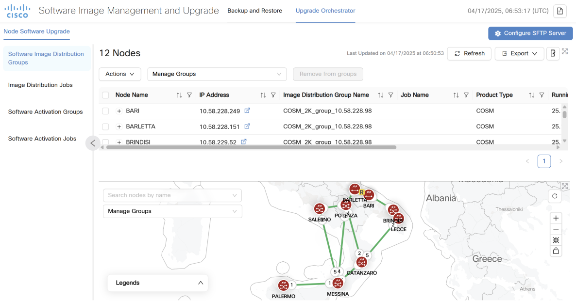
Figure 65: Upgrade Orchestrator
