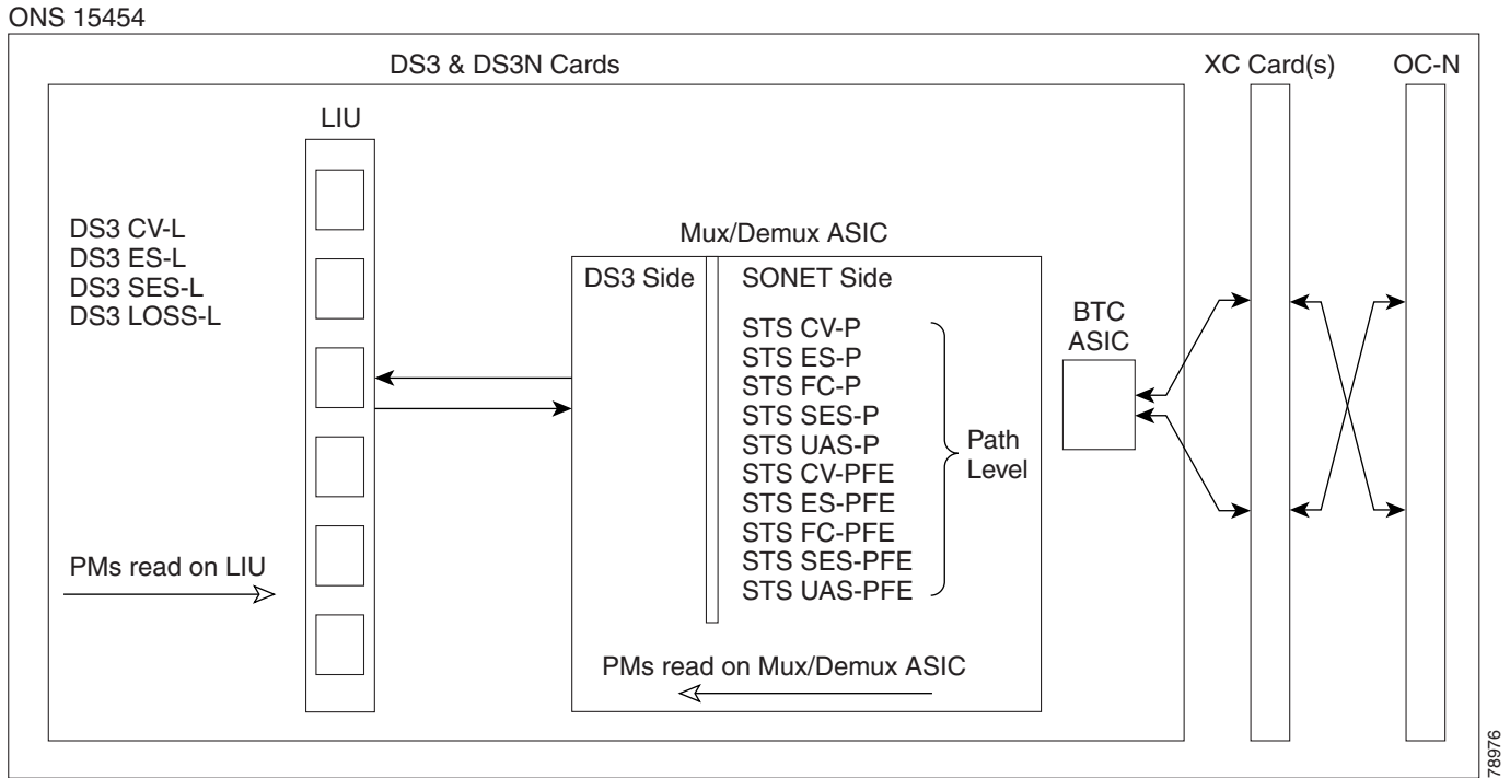
Figure 15-9 PM Read Points on the DS3-12 and DS3N-12 Cards
