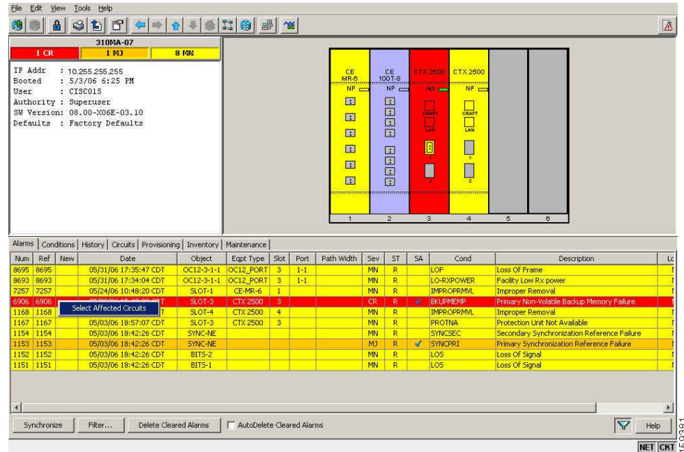
Figure 11-1 ONS 15310-MA Select Affected Circuits Option
