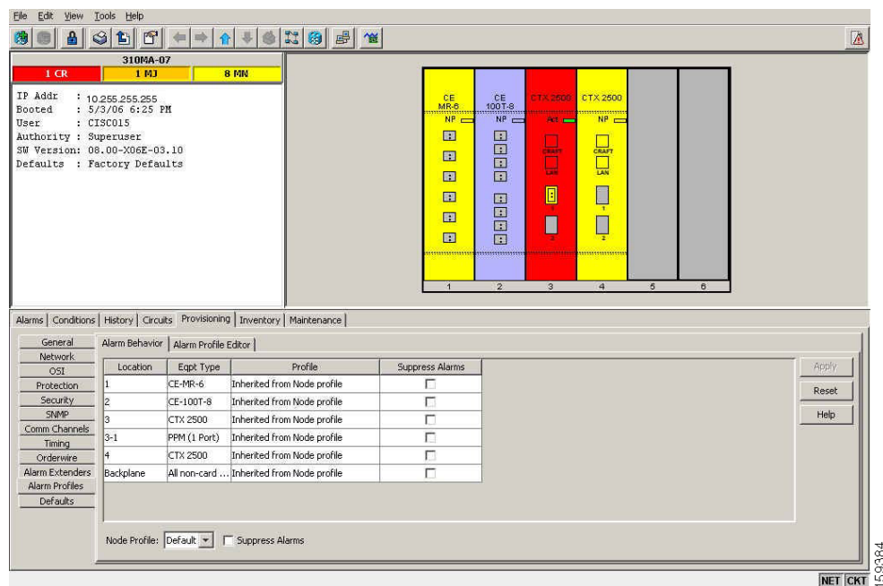
Figure 11-2 Alarm Profile for a 15310-MA CTX2500 Card
