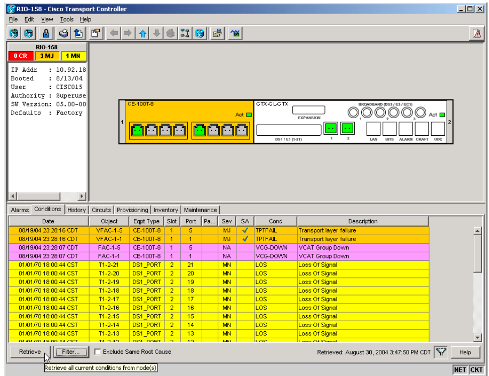
Figure 6-1 Node View Conditions Window
