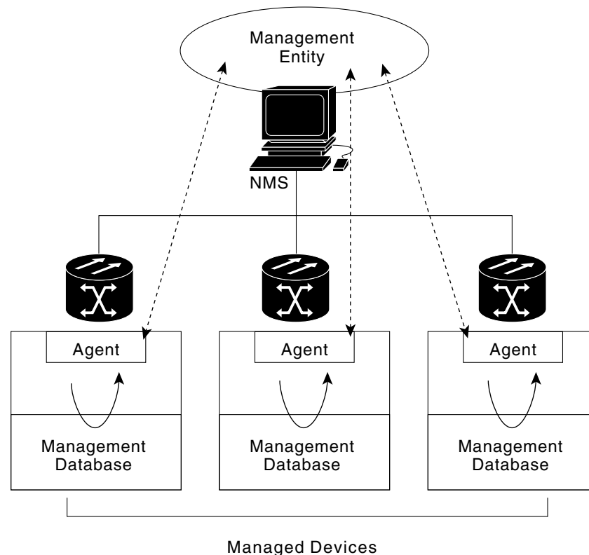
Figure 14-3 Example of the Primary SNMP Components
