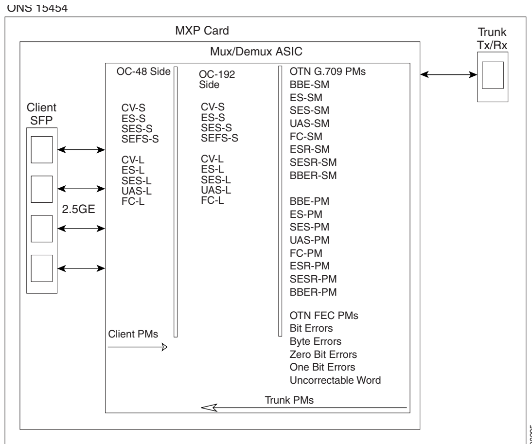
Figure 12-20 PM Read Points on MXP-2.5G-10G Cards
