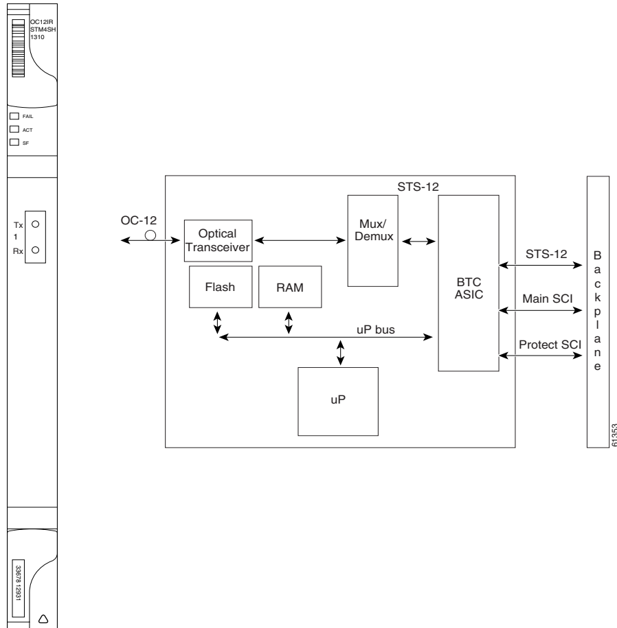
Figure 4-4 OC12 IR/STM4 SH 1310 Faceplate and Block Diagram
