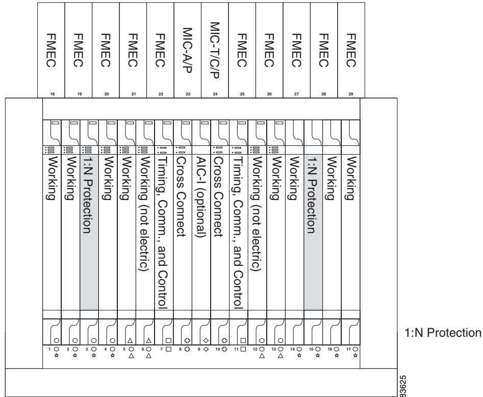
Figure 6-3 ONS 15454 SDH Cards in a 1:N Protection Configuration
