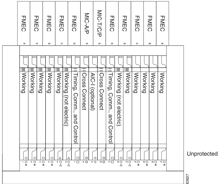
Figure 6-1 ONS 15454 SDH Cards in an Unprotected Configuration
