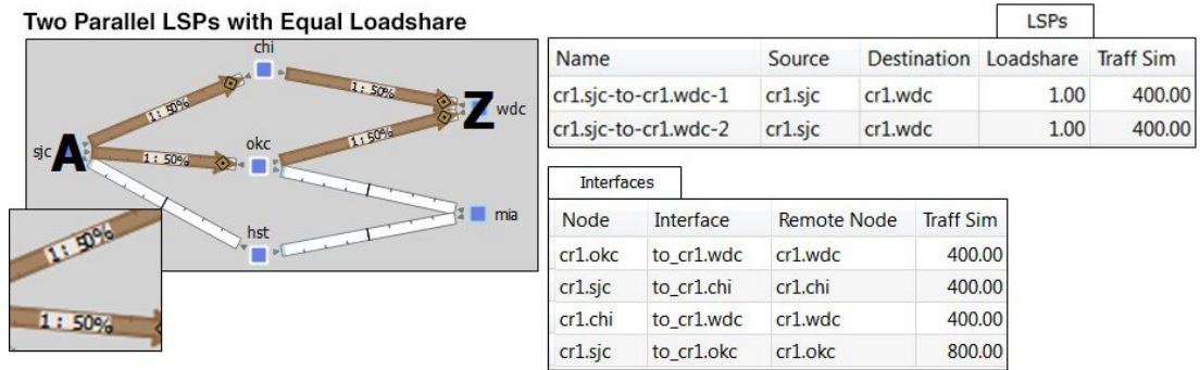
Figure 3: Example of Two Parallel LSPs with Equal Loadsharing
