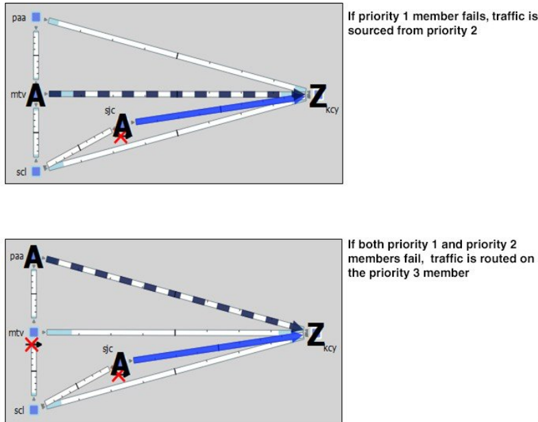
Figure 3: Example Failover for Multiple Data Centers
