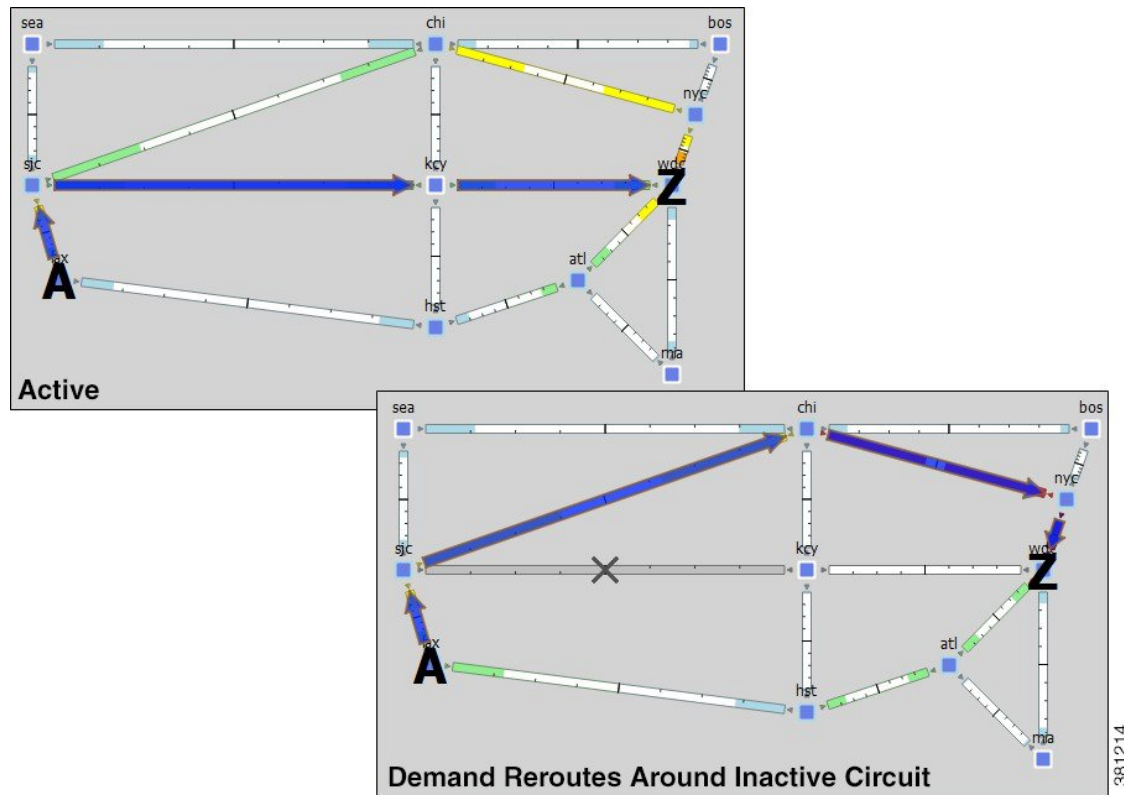
Figure 3: Inactive Circuit
