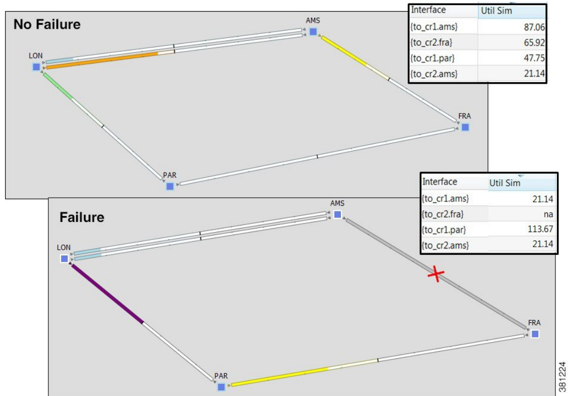
Figure 1: Failed Circuit
