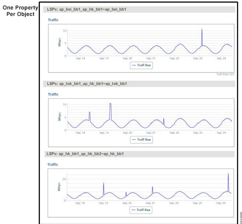
Figure 2: Example of Graphing Individual Objects
