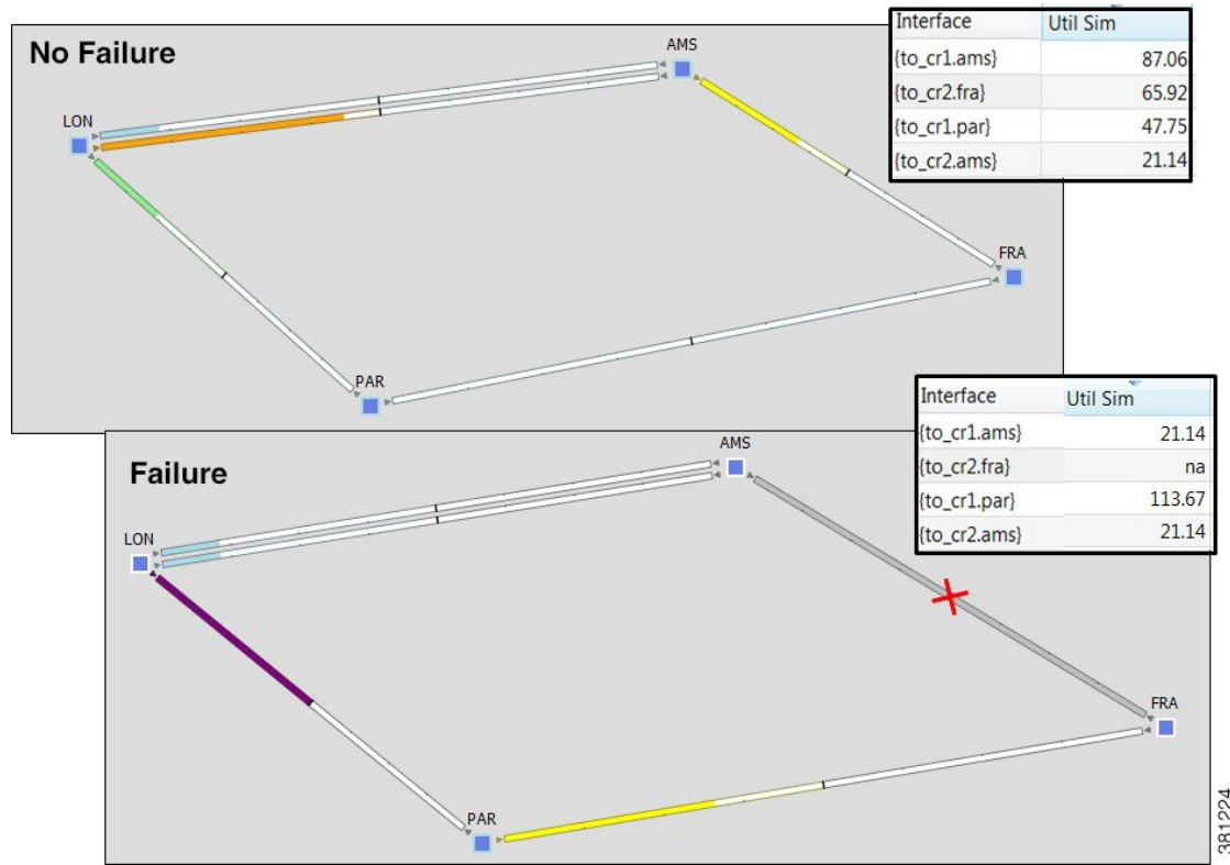
Figure 1: Failed Circuit
