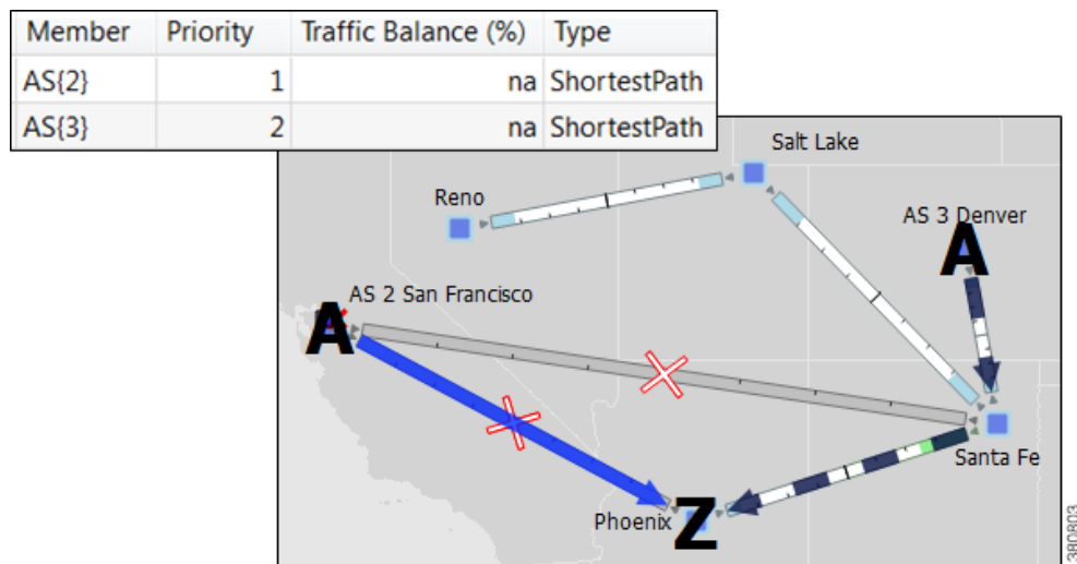
Figure 16-7 Example Failover to a Different External AS
