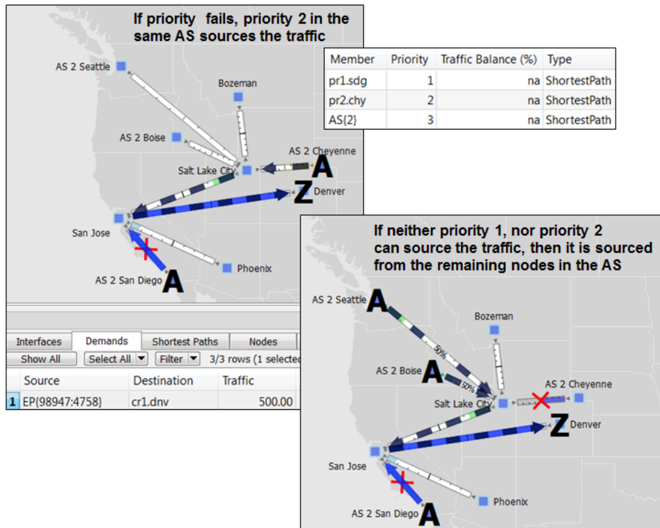
Figure 16-5 Example Failover Within the Same External AS
