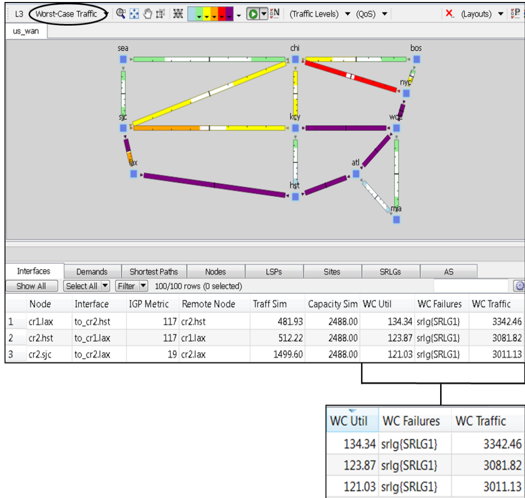
Figure 3-3 Worst-Case Simulation
