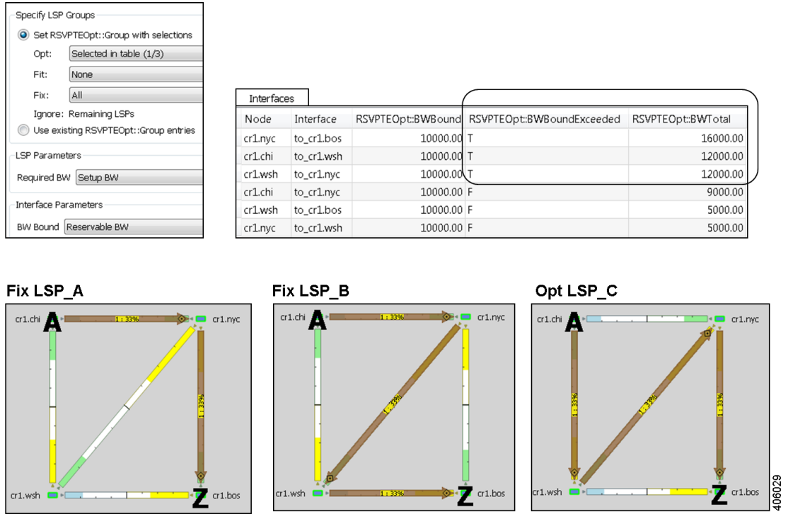
Figure 19-6 Example: Congestion Occurs When Settings LSPs to Fix
