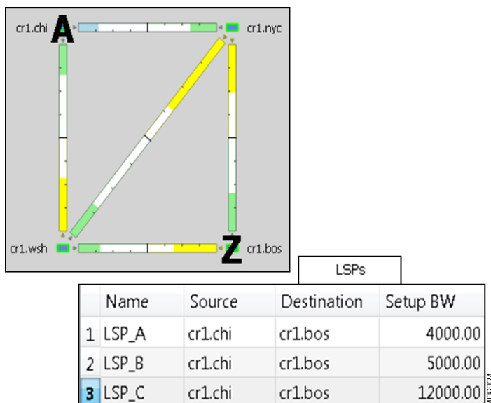
Figure 19-5 Unroutable LSP Due to Insufficient Bandwidth
