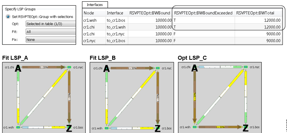
Figure 19-7 Example: Tactical Congestion Mitigation Using Fit LSPs
