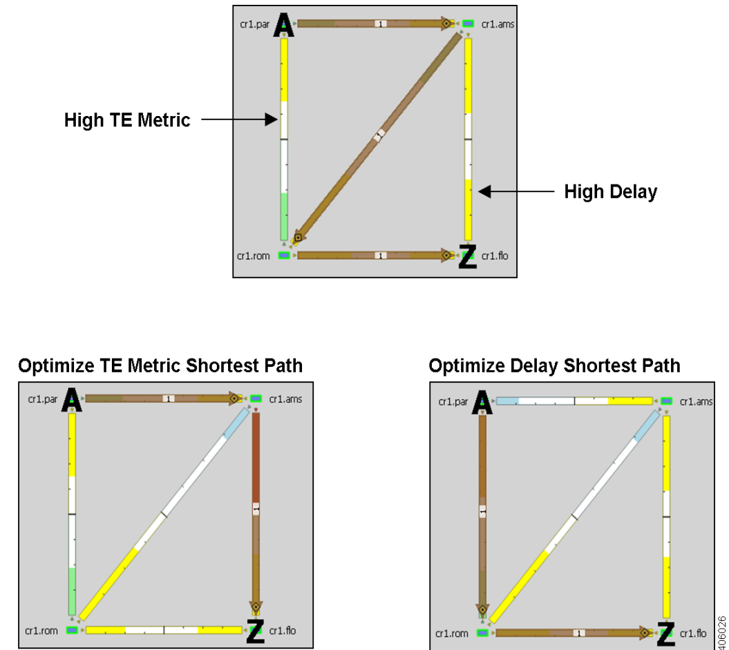
Figure 19-1 Example Shortest Path Optimization
